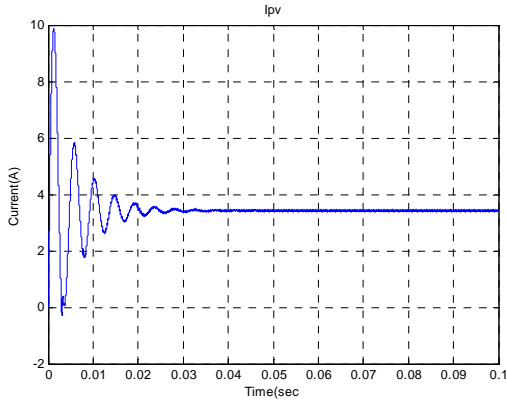
Figure 17. The output PV panel current
