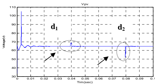
Figure 26. The output PV panel voltage with the occurrence of two solar irradiance disturbances
