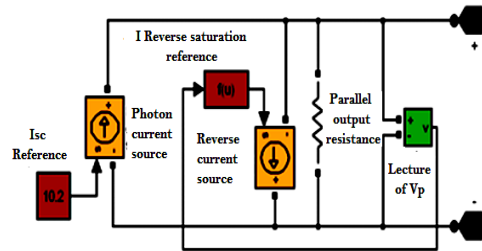
Figure 4. Photovoltaic solar modelled with Malab/Simulink
