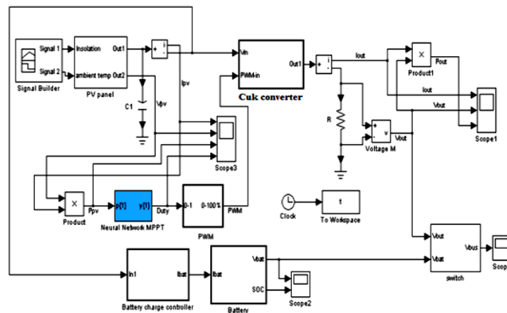
Figure 16. Simulation system in MATLAB/Simulink
