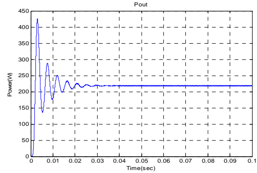
Figure 22. The Cuk converter output power with The ANN controller
