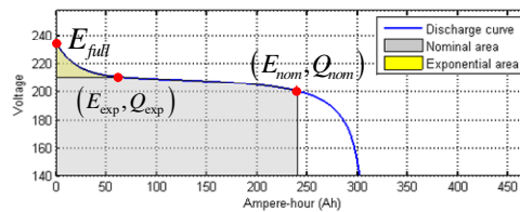
Figure 12. Discharge characteristics curve of the battery at the rated discharge current (V-Q)
