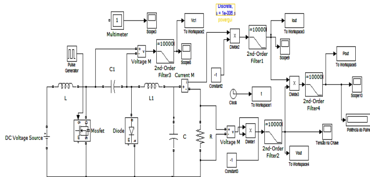
Figure 10. Matlab/Simulink simulation model of the Cuk converter
