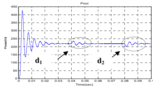
Figure 31. The Cuk converter output power with two disturbances
