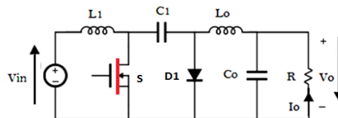
Figure 7. Cuk converter
