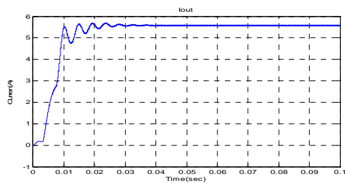
Figure 36. The Cuk converter output current with a step change of irradiance
