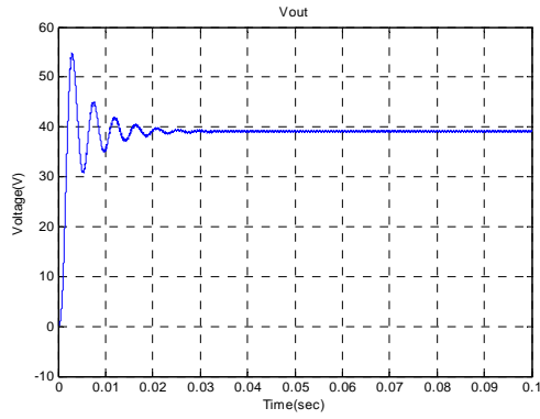
Figure 21. The Cuk converter output voltage with The ANN controller
