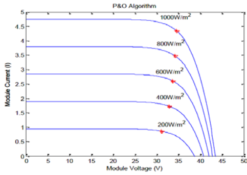
Figure 5. Characteristic curves current of solar panel, at different irradiance levels and 25°C
