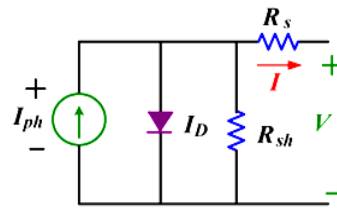
Figure 3. Equivalent circuit of a solar cell
