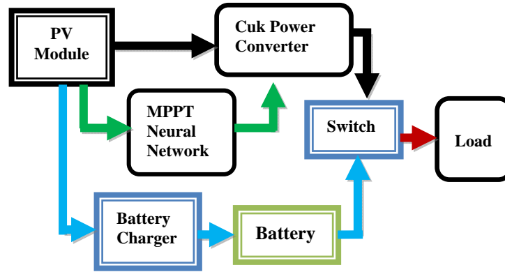
Figure 1. Outline of the proposed system
