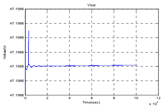
Figure 23. The output battery voltage during charging Period
