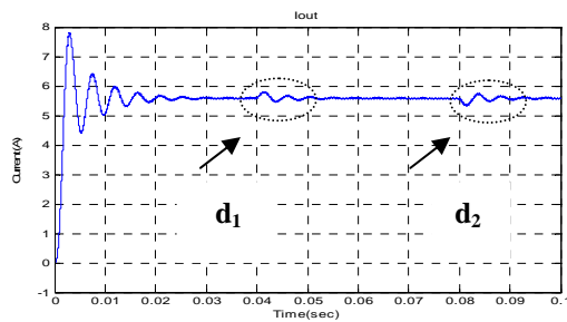
Figure 28. The Cuk converter output current with the occurrence of the two disturbances
