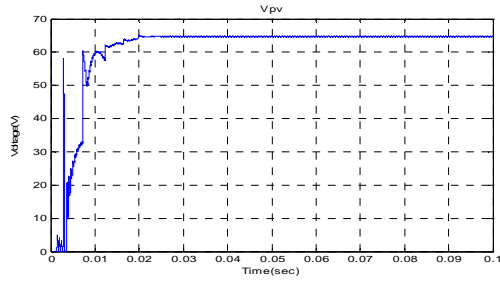
Figure 34. The output PV panel voltage with a step change of irradiance
