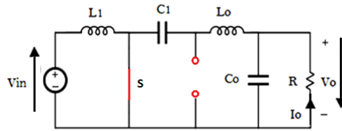
Figure 8. Cuk converter on state
