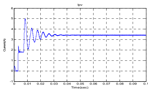
Figure 33. The output PV panel current with a step change of irradiance
