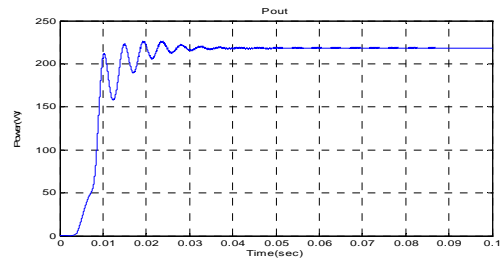
Figure 38. The Cuk converter output power with a step change of irradiance
