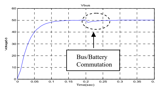
Figure 32. The output load voltage during the bus/battery commutation
