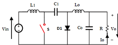
Figure 9. Cuk converter in the off-state
