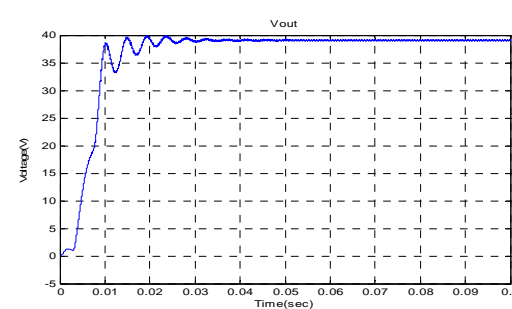
Figure 37. The Cuk converter output voltage with a step change of irradiance
