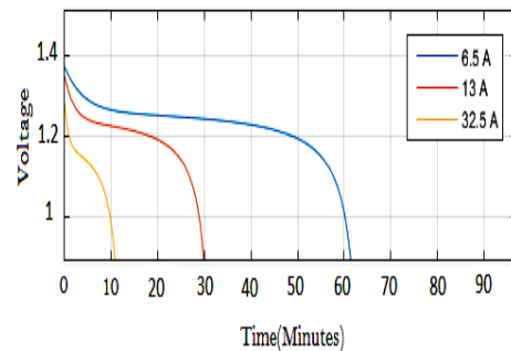
Figure 14. Discharge characteristics curves of the battery at different discharge current (V-Q)
