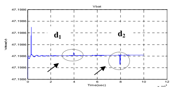
Figure 30. The output battery voltage with two disturbances during the Charging Period
