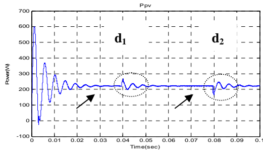
Figure 27. The output PV panel power with the occurrence of the two disturbances
