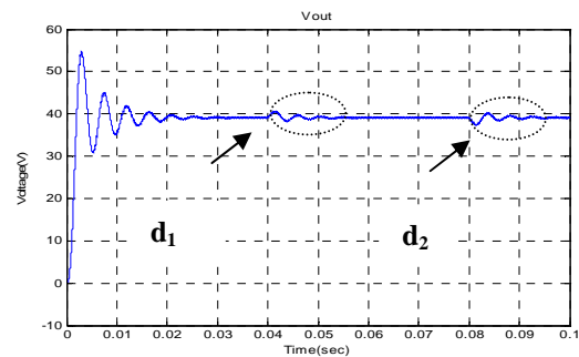
Figure 29. The Cuk converter output voltage occurrence of two solar irradiance disturbances
