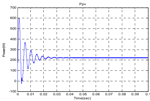
Figure 19. The output PV panel power
