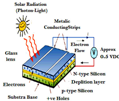
Figure 2. Basic structure of a PV cell
