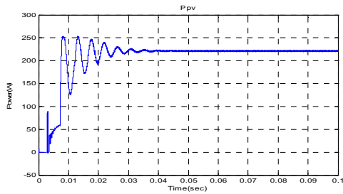
Figure 35. The output PV panel power with a step change of irradiance
