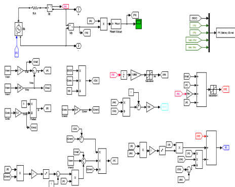
Figure 13. The battery model in MATLAB/Simulink
