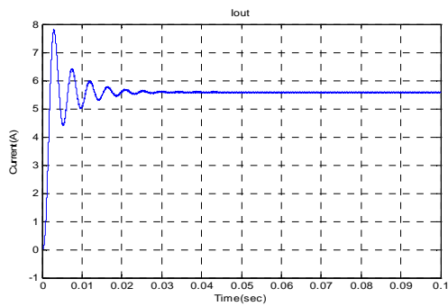
Figure 20. The Cuk converter output current with ANN controller
