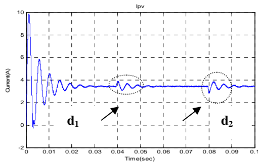
Figure 25. The output PV panel current with the occurrence of the two disturbances
