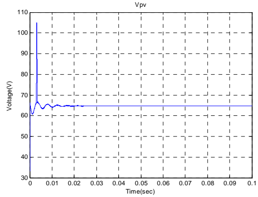
Figure 18. The output PV panel voltage
