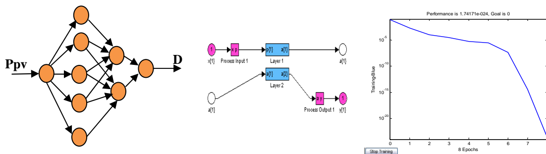
Figure 15. Training error using the neural network MLP
