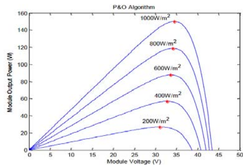
Figure 6. Characteristic curves power of solar panel, at different irradiance levels and 25 °C
