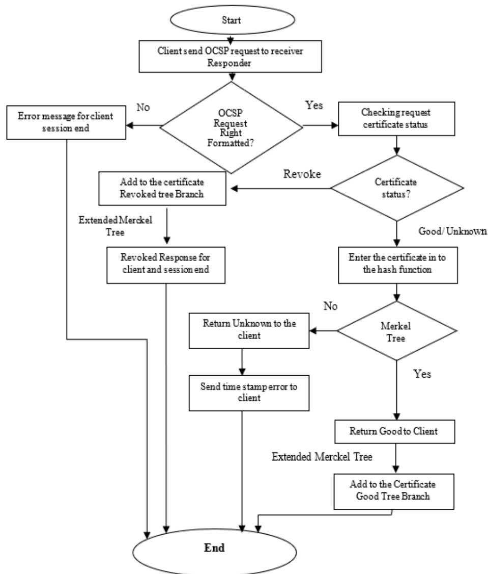
Figure 5. Proposed flowchart of OCSRP responder to verify certificates using extended Merkle's tree, works on sorting certificates out in different cases
