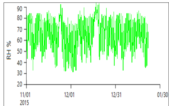
Figure 6. Reference Building Indoor Humidity Level
