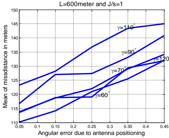
Figure 8. Mean of miss Distance variation with antenna positioning angular error (without additive noise) at L=600\text{meter}, J/S=1, \gamma=60^\circ to 120^\circ; R_t=10\text{Km}
