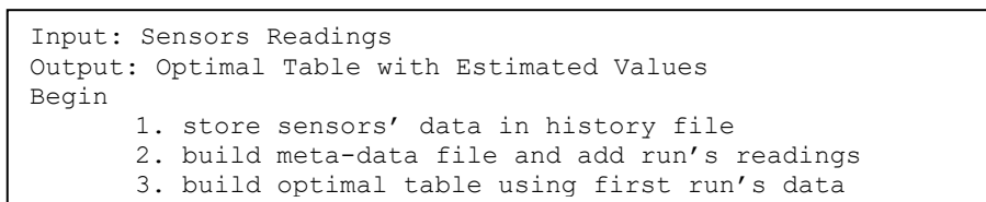
Figure 2. Algorithm for the first treatment run
