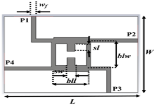
Figure 1. The proposed design of 5G coupler (top view)
