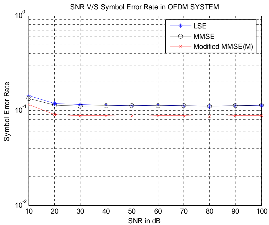
Figure 6. Performance comparison of 32QAM symbol error rate.
