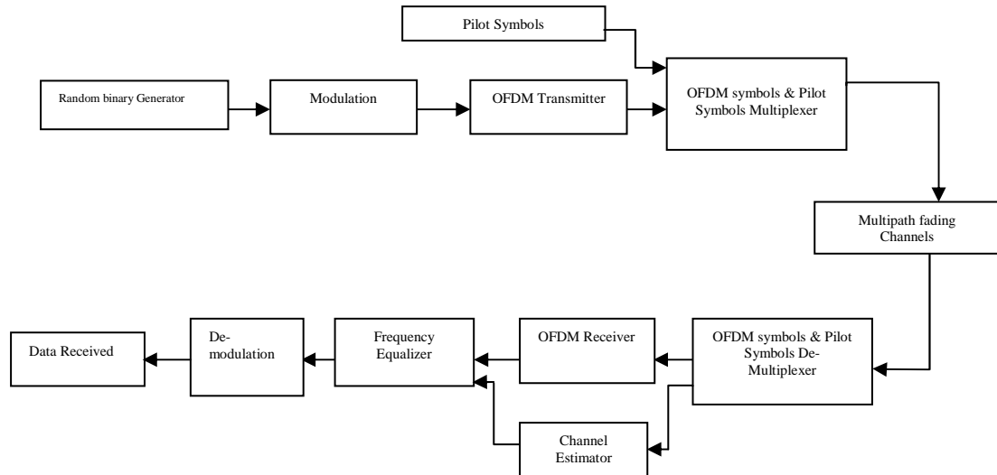
Figure. 1 OFDM system block diagram
