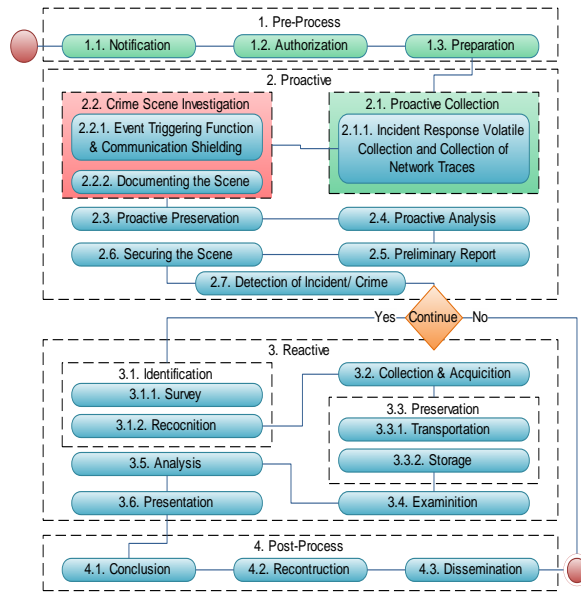
Figure 6. IDFIF v1 for smartphone investigation [7-8]
