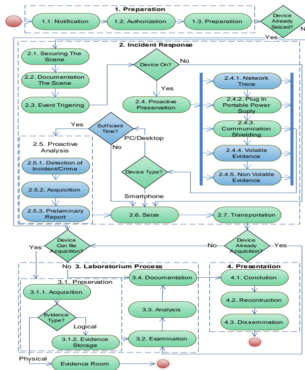
Figure 7. IDFIF v2 for smartphone investigation
