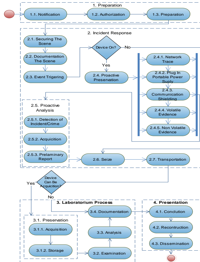
Figure 4. Conceptual IDIFIF v2
