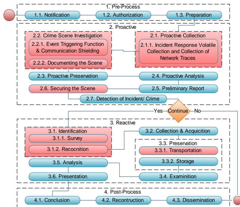
Figure 3. Rich picture IDFIF [7-8]
