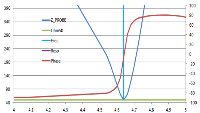
Figure 8. impedance of probe vs frequency. horizontal axis is frequency in MHz, vertical axis in left is Z probe in ohms, vertical axis in right is phase in degrees
