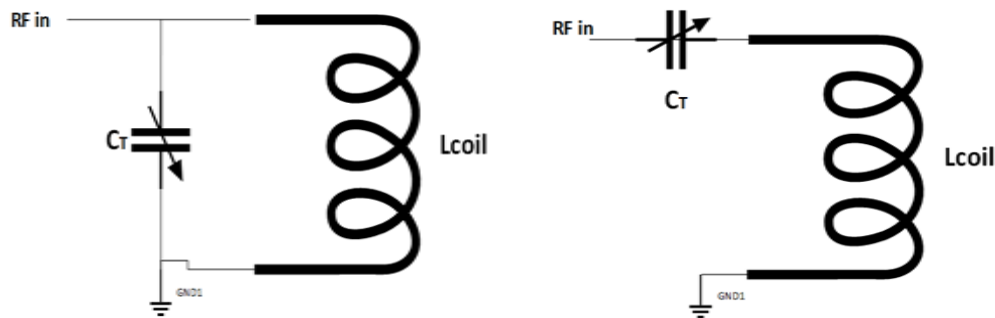
Figure 2. The parallel and series LC probe
