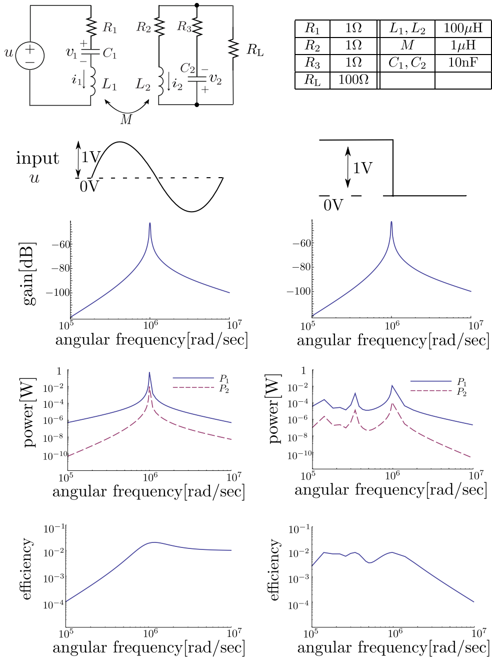
Figure 4. Bode diagram and power and efficiency with a parallel circuit
