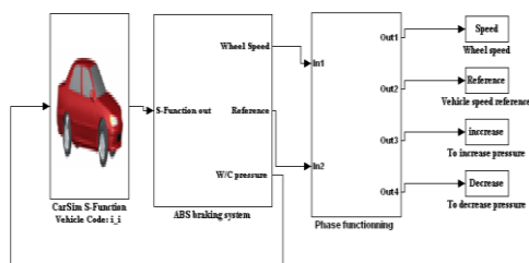
Figure 5. Simulink-CarSim model of the ABS system
