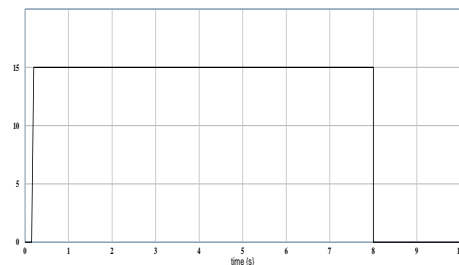
Figure 6. Brake set point on the master cylinder
