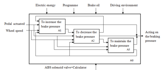
Figure 3. Node A0 of the SADT model
