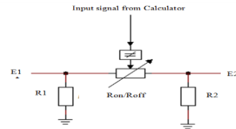
Figure 12. Equivalent circuit of an On/Off switch
