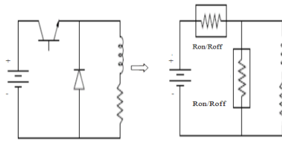
Figure 11. Fixed topology of a diode
