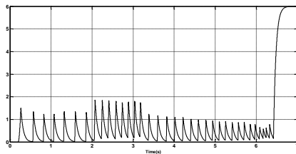
Figure 9. Pressure evolution applied to the brake disc during the braking operation
