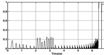
Figure 10. Slip coefficient evolution during braking
