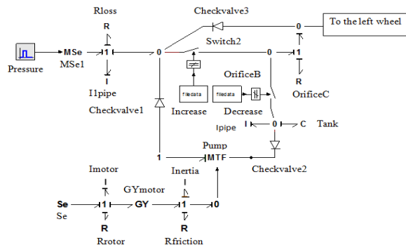
Figure 13. The bond graph model of the hydraulic system controlled by a calculator
