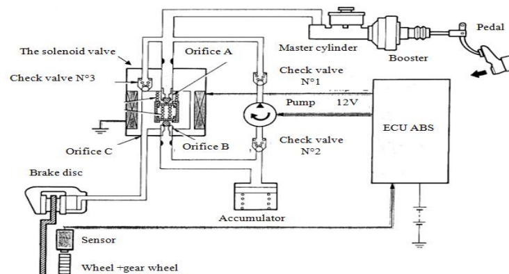
Figure 1. Elements of the ABS system
