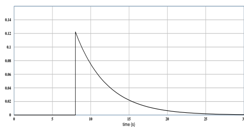
Figure 16. Oil flow rate, check valve 3
