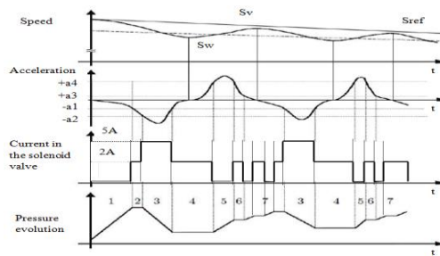
Figure 4. Operating strategy of the ABS calculator
