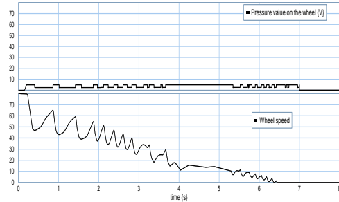
Figure 15. Pressure variation as a function of the speed of the left wheel
