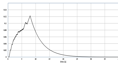
Figure 17. Flow variation in the pipeline
