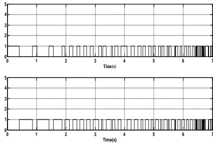
Figure 14. Calculator control signals during braking
