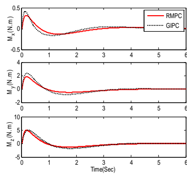
Figure 4.b. Control actions comparison between the RMPC and GIPC algorithms without constraint
