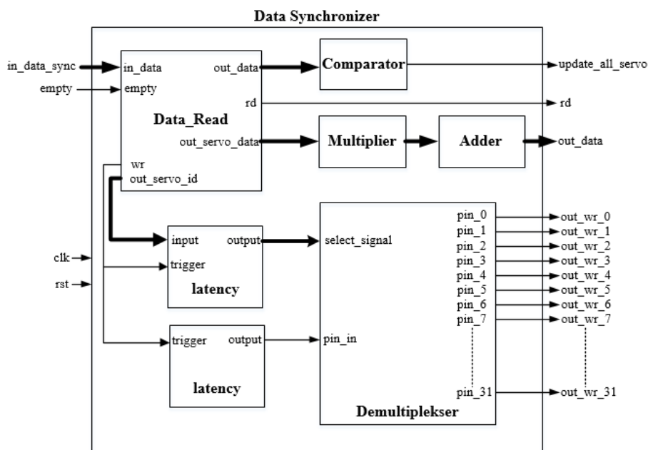
Figure 5. Block diagram of data synchronizer module
