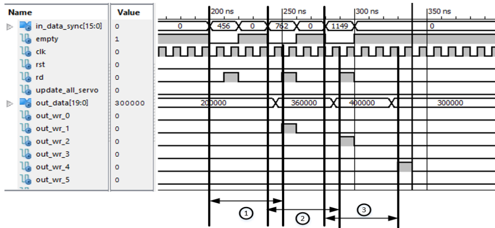
Figure 10. Simulation result of data synchronizer
