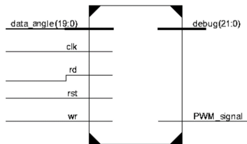
Figure 6. Module of PWM generator
