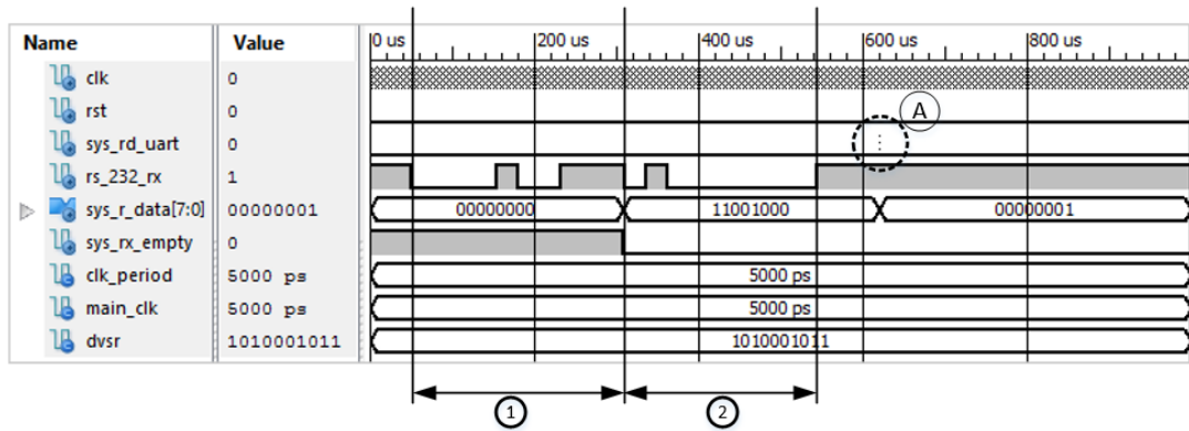
Figure 8. Simulation result of serial receiver module
