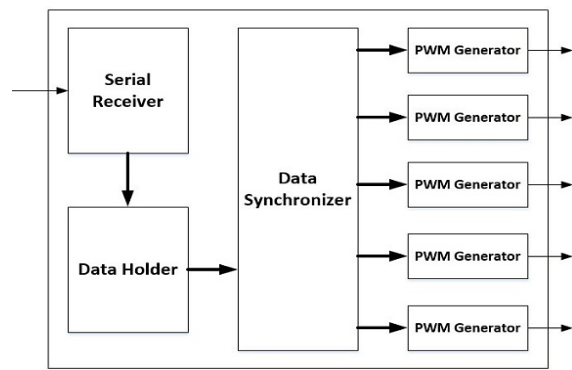
Figure 2. Block diagram of FPGA system
