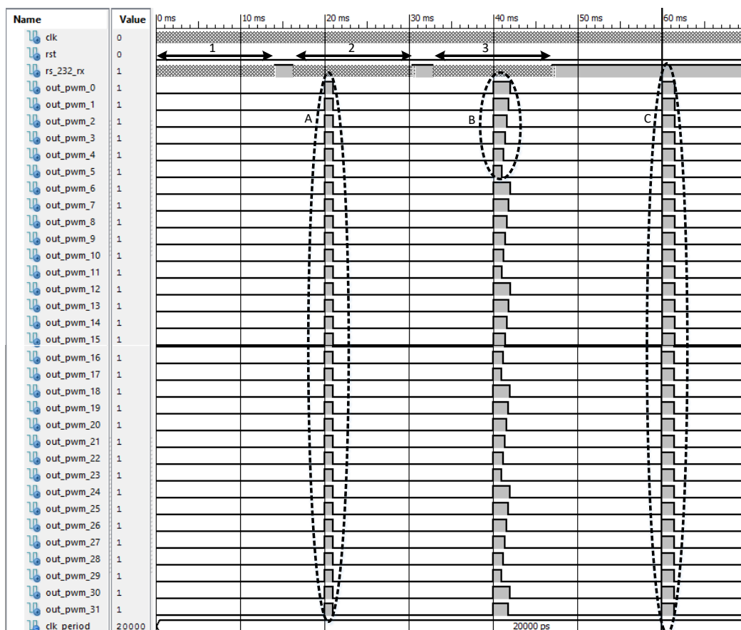
Figure 12. Simulation result of overall system
