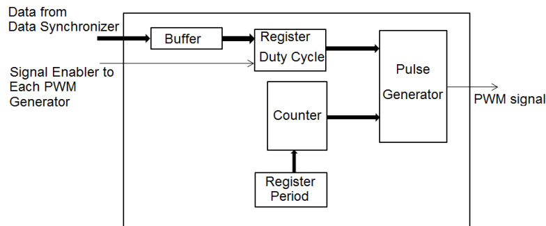
Figure 7. Module of PWM generator
