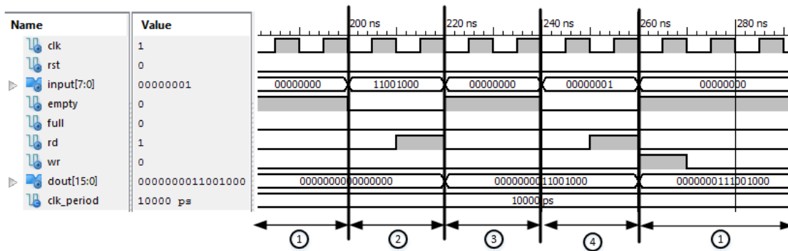
Figure 9. Simulation result of data holder module
