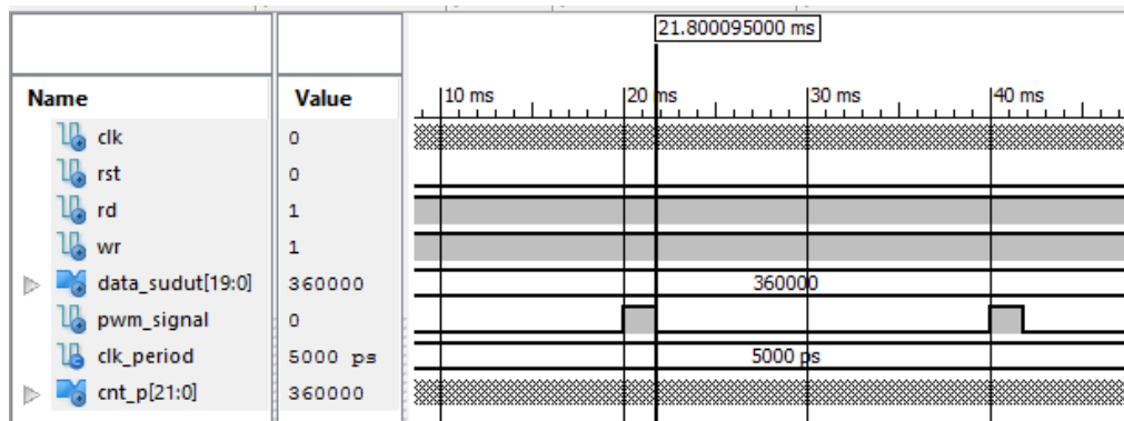
Figure 11. Simulation result of PWM generator
