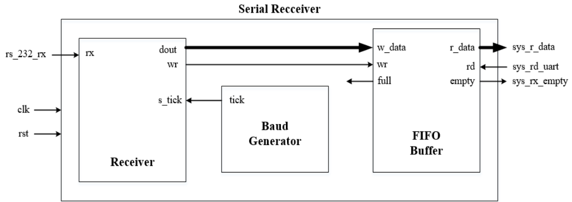
Figure 3. Block diagram of serial receiver module
