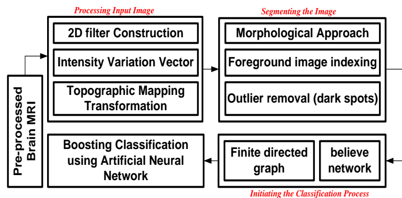
Figure 1. Undertaken scheme of proposed classification
