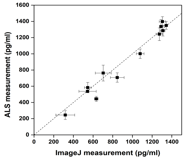
FIGURE 6. Comparison curve between the measured values of 12 LFIA patient samples, as measured using ImageJ image analysis from a scanned image, and the biomarker analyser ALS-based measured value.
