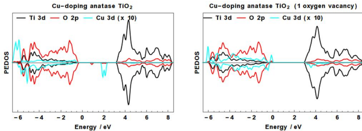
Figure 7: Hybrid DFT PEDOS for Cu-doped TiO 2 . Left panel: Cu-doped anatase with no compensating oxygen vacancy, right panel: Cu-doped anatase with the compensating oxygen vacancy.
