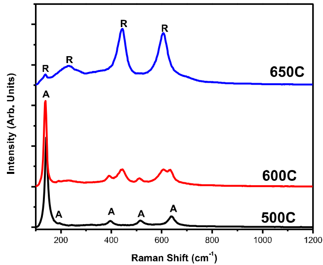
Figure 3: Raman spectra of 0% Cu-doped TiO 2 .
