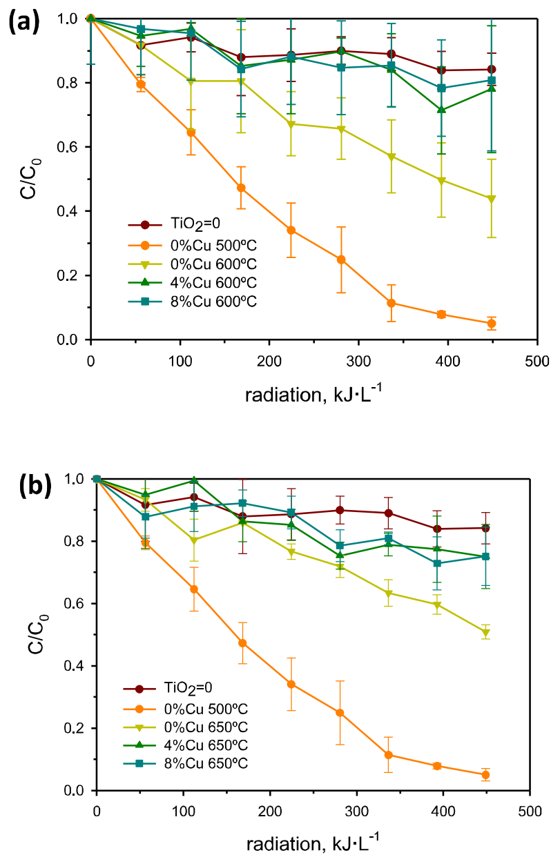
Figure 8: Degradation of 1,4-dioxane by Cu-doped \text{TiO}_2 photocatalysis at (a) 600°C and (b) 650°C compared with \text{TiO}_2 prepared at 500°C and radiation without catalyst.
