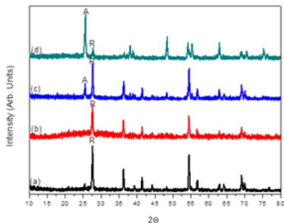
Figure 1: XRD of (a) 0% Cu-TiO 2 (b) 2% Cu-TiO 2 (c) 4% Cu-TiO 2 (d) 8% Cu-TiO 2 after calcining to 650°C. A = anatase and R = Rutile
