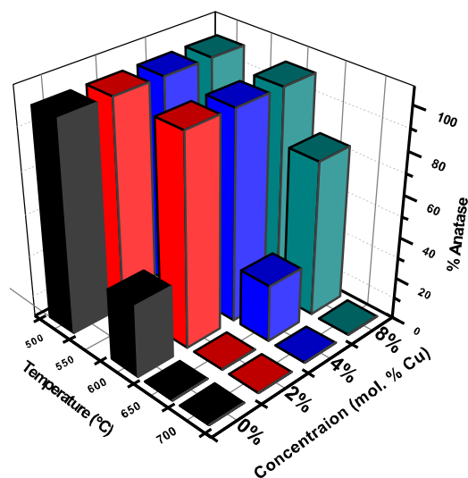
Figure 2: Percentage of the anatase phase in Cu-doped TiO 2 samples
