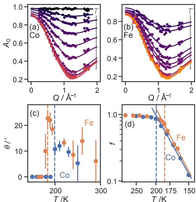
Fig. 2 Fitted elastic incoherent structure factors A_0 for (a) \mathbf{M} = \text{Co} , (b) \mathbf{M} = \text{Fe} . (c) Fitted values of the tilt angle \theta for \mathbf{M} = \text{Co} (blue) and \text{Fe} (orange). Error bars are not meaningful when this angle refines to zero and are therefore not shown in this case. (d) Arrhenius plot of fraction f of molecules rotating (logarithmic scale) as a function of temperature (inverse scale). In (c) and (d), the nominal IT-HT phase transition temperatures are shown as dashed lines.
