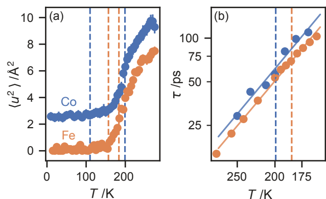
Fig. 3 (a) Mean-square deviation of atomic positions as a function of temperature. (b) Arrhenius plot of the correlation time \tau (logarithmic scale) as a function of temperature (inverse scale). Nominal phase transition temperatures are shown as dashed lines.
