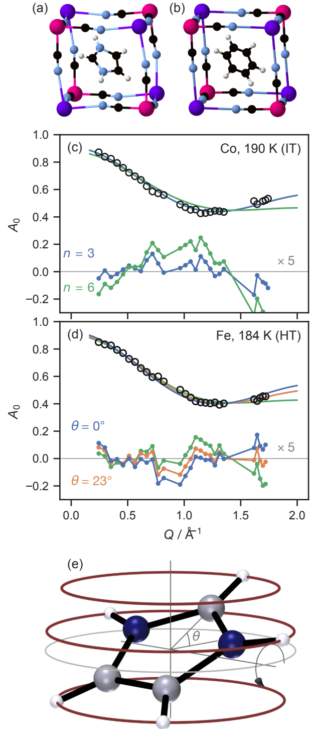
Fig. 1 Crystallographic structures of the target materials in (a) LT; (b) IT and HT phases. The “benzene” molecule represents the imidazolium ion disordered about the threefold axis. Representative elastic incoherent structure factors A_0 for (c) \mathbf{M} = \text{Co} , IT phase; (d) \mathbf{M} = \text{Fe} , HT phase. A model with a sixfold rotation axis (green) gives a poor fit in both phases. A model with a threefold rotation axis and no tilt of the imidazolium ion (blue) fits well in the IT phase, but not in the HT phase. Allowing the tilt angle \theta to refine (orange) improves the fit in the HT phase. Gaps in Q occur where Bragg peaks have been omitted from the data. (e) Tilting model. If the plane of the imidazolium ion is tilted by \theta with respect to the rotation axis, different H atoms rotate with different effective radii (red circles), of which some or all are smaller than the untilted value (grey circle).
