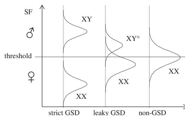
Figure 2. Threshold model of sex determination. An individual develops as male if the expression of the sex factor (SF) exceeds a given threshold, and as female otherwise. Strict GSD results if all XY individuals, but none of the XX, exceed the threshold (left). Leaky GSD results if XY and XX distributions overlap somewhat (centre). Non-GSD results if a single genotype (XX) occurs; individual sex is then determined by random noise in the expression of the sex factor (right).
