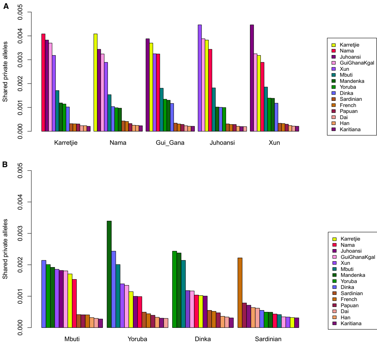
Fig. 2. Grouped bar-plots summarizing private allele sharing as a fraction of the total number of variant sites in the data set: (A) Privately shared alleles of various Khoe-San groups with comparative groups. (B) Privately shared alleles of comparative groups.
