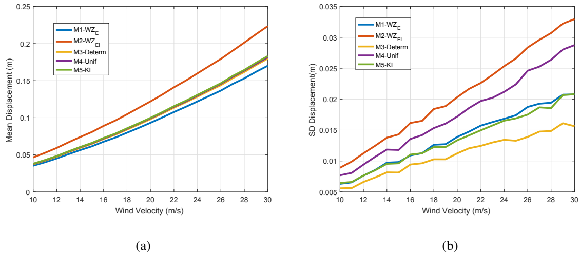
Figure 3: Top displacement of the pole. a) Mean displacements; b) SD displacements.
