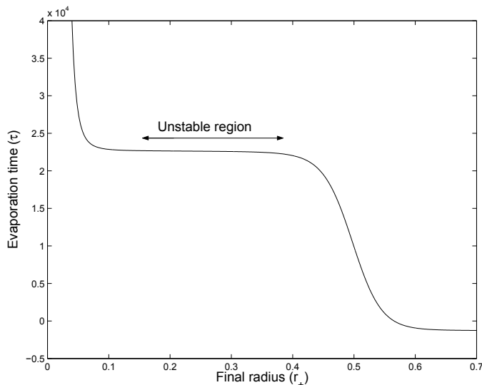
FIG. 5: Evaporation time \tau as a function of the final radius r_+ [ \alpha = 0.05 , e = 1 , b = 2 ]. A plateau manifestly appears in the evaporation rate. The graph has been normalized by means of an appropriate redefinition of the Stefan-Boltzmann constant.
