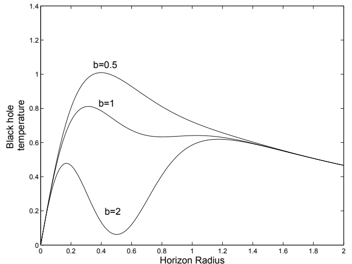
FIG. 4: Black hole temperature as a function of the horizon radius [ \alpha = 0.05 , e = 1 ]; representing the caloric curve.
