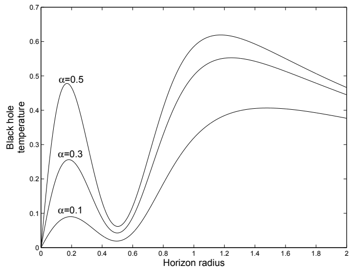
FIG. 3: Black hole temperature as a function of the horizon radius [ b = 2 , e = 1 ]; representing the caloric curve.
