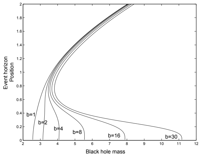
FIG. 1: The position of the event horizon as a function of the black hole mass for different values of b [ \alpha = 0.5 , e = 1 , \Lambda = 0 ].
