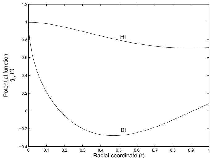
FIG. 2: The (potential) function g_\alpha(r) for both Hoffmann-Infeld (HI) and Born-Infeld (BI) solutions [ \alpha = 0.1 , e = 1 , \Lambda = 0 ].
