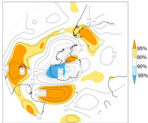
c) ERI PNM, DEFMAM
