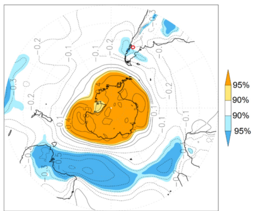
c) ERI PNM, DEFMAM
