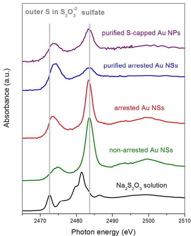
34 Figure 4: S-K XANES spectra of the different samples: reference thiosulfate solution 35 (black); non-arrested Au NSs (green); non-purified arrested Au NSs (red); purified 36 arrested Au NSs (blue) and purified S-covered Au NPs used as a reference (violet). 40 41 42 43 44 45 46 47 48 49 50 51 52 53 54 55 56 57 58 59 60
