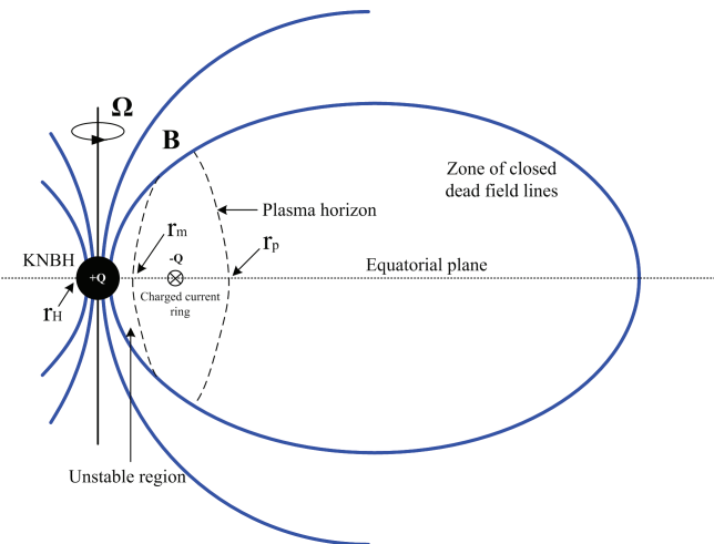
FIG. 1.— Schematic diagram of the initial state of a KNBH.
