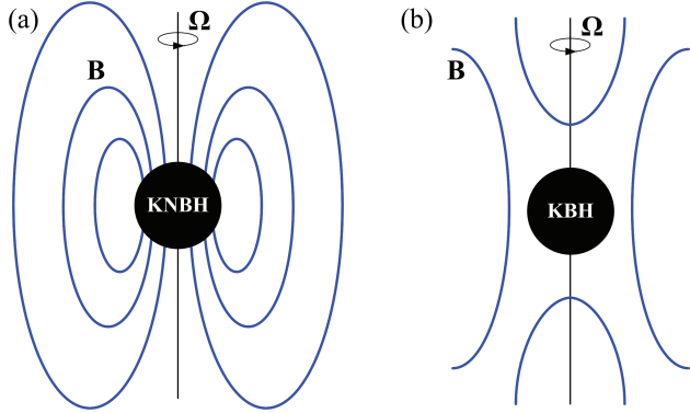
FIG. 4.— Schematic diagram of the magnetic field configuration during the discharging of a KNBH in a binary.
