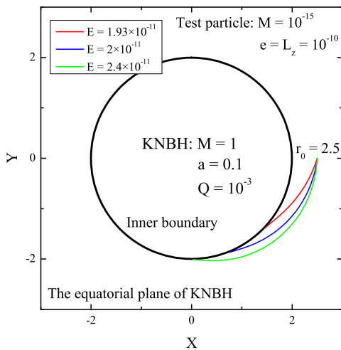
FIG. 3.— The trajectories of a test particle ( m = 10^{-15} , and e = L_z = 10^{-10} ) on the equatorial plane falling into a KNBH ( M = 1 , a = 0.1 , and Q = 10^{-3} ) from r_0 = 2.5 to the inner boundary ( r = r_g ) for E = 1.93 \times 10^{-11} , 2 \times 10^{-11} , and 2.4 \times 10^{-11} .
