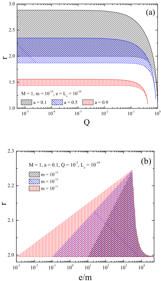
FIG. 2.— Unstable region on the equatorial plane ( r_H < r < r_m ) around a KNBH ( M = 1 ) as functions of the KNBH spin and charge (panel a) with m = 10^{-15} and e = L_z = 10^{-10} , and the specific charge of the particle (panel b) with a = 0.1 , Q = 10^{-3} , and L_z = 10^{-10} .
