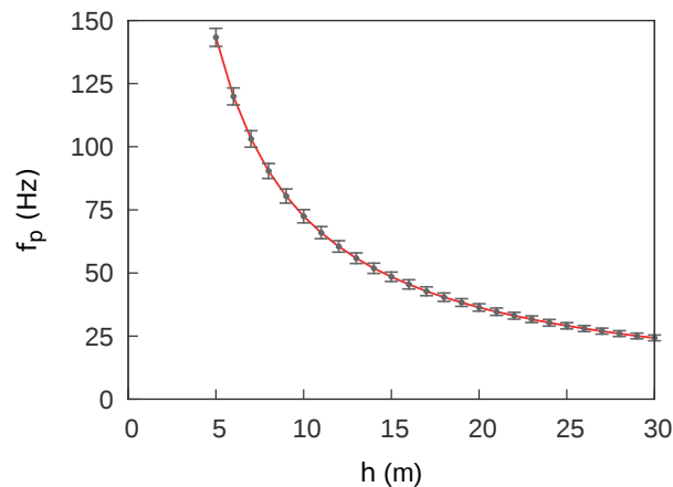
Figure 7: Average peak frequency \bar{f}_p versus layer thickness h . Each point is an average over the \text{CO}_2 overall saturation \bar{S}_g range between 10% to 90%. The vertical lines show the dispersion of the mean value, which increases as layer thickness becomes thinner.
