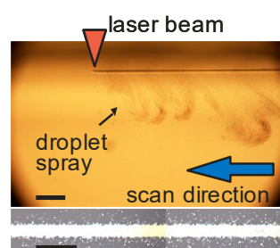
Figure 3. Image of the spray ejection during CW-LIFT of a silver nanoparticle ink at a laser power density of 13 kW/cm 2 and a scan speed of 300 mm/s. The donor film is in the top of the picture. The laser impinged from above, scanning from right to left. The laser spot position when the picture was taken is indicated with red arrow. Below, an image of a conductive line printed under the same conditions with the receiving substrate placed at 150 μm. Scale bars are 500 μm in both pictures. Readapted from [26] under Creative Commons license.
