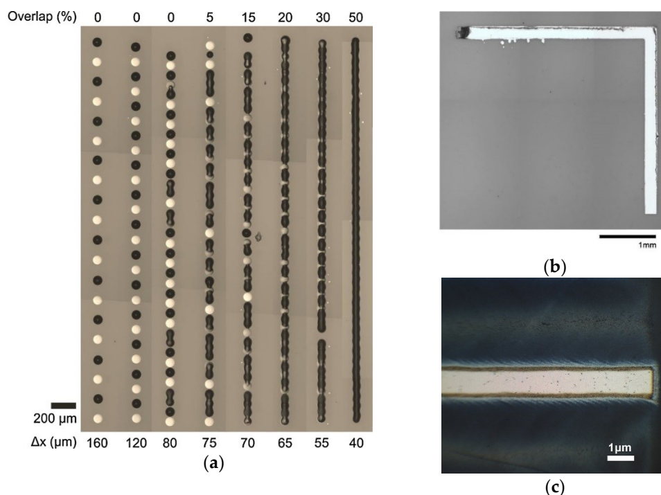
Figure 5. Optical microscopy images of: (a) Lines of droplets printed in alternate sequence with different overlaps ( \Delta x is measured from center to center). Dried droplets appear as bright spots. [72]. (b) Conductive ink printed on fluidic guides forming an angle of 90^\circ [75]. (c) Ag conductive line printed on PEN substrate after laser sintering and patterning by laser ablation [73]. Reprinted from [72], [75], and [73], respectively, with permissions of Elsevier.
