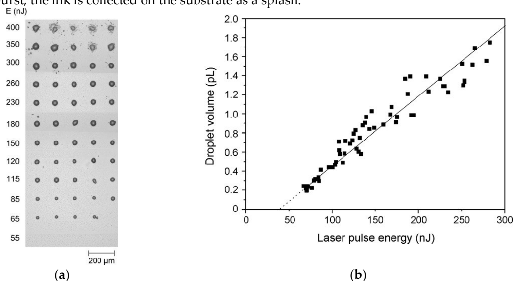
Figure 4. (a) Optical microscopy image of droplets printed by LIFT at different laser pulse energies (indicated on the left of each row). (b) Plot of the volume of the droplets printed in (a) vs. the laser pulse energy. Reprinted from [31] with permission of Elsevier.
