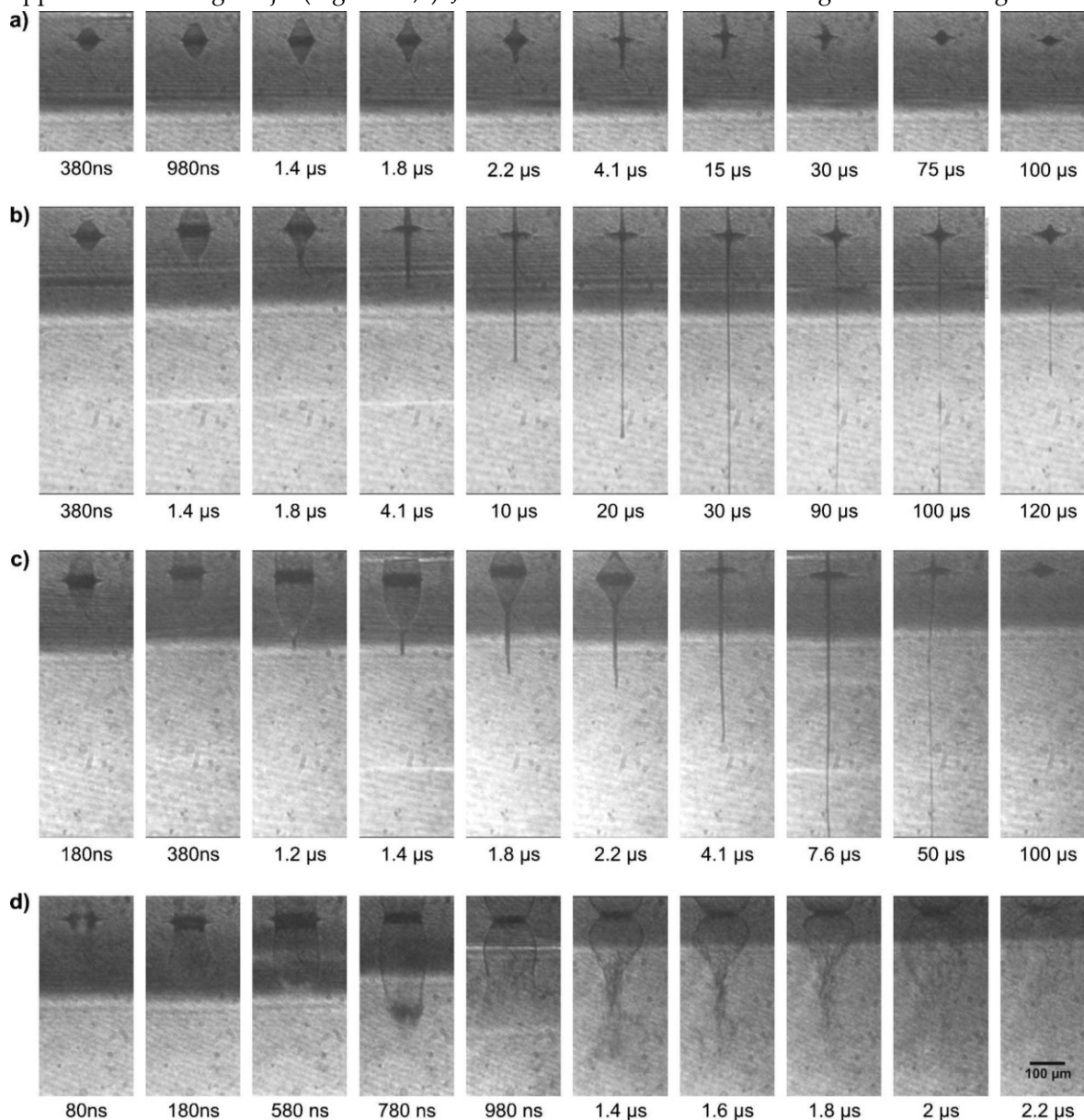
Figure 2. Images of a time resolved study of liquid ejection in LIFT at different laser fluences (a) 1.2, (b) 2.4, (c) 5.6, and (d) 10 J/cm 2 . The delay time with respect the laser pulse is indicated on top of each image. The laser beam impinges the donor layer from the top of the image. Reprinted from [37] with permission of AIP Publishing.
