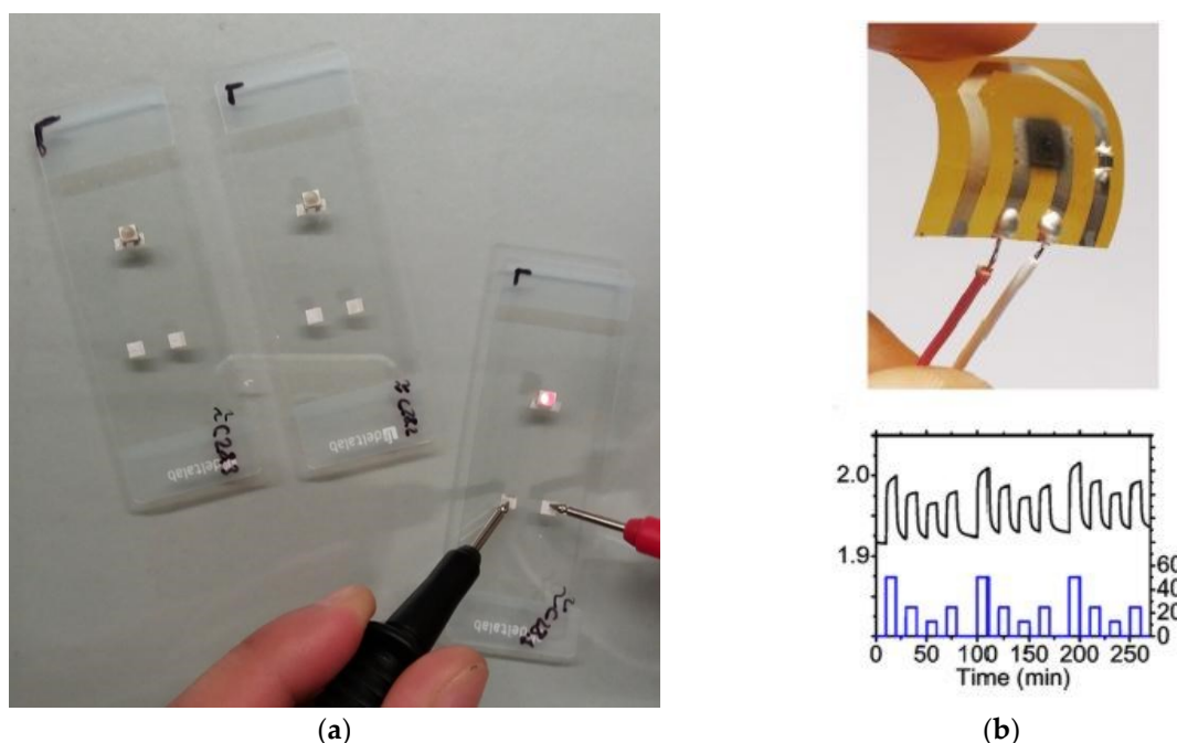
Figure 7. (a) Image of circuits with two invisible electrodes of Ag nanowires printed by LIFT on glass. The injection of current provokes LED illumination for confirming the conductivity of the tracks. Reprinted from [122] with permission of Elsevier. (b) Image of a humidity sensor with carbon nanofibers printed by LIFT on a flexible substrate and dynamic response of the sensor (black) to humidity changes (blue). Reprinted with permission from [25]. Copyright (2017) American Chemical Society.
