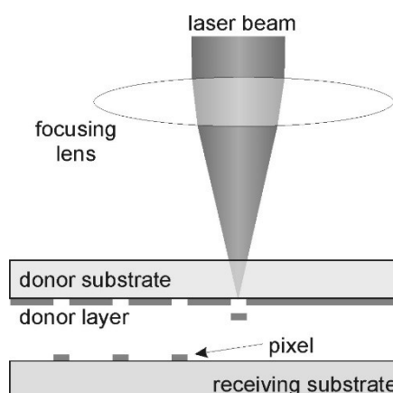
Figure 1. Scheme with the main elements in a typical Laser-induced forward transfer (LIFT) setup for laser printing.
