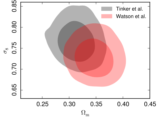
Fig. A.2. Robustness to the choice of mass function. The grey shaded contours give the cosmological constraints when using the Tinker et al. (2008) mass function, corresponding to our final result. This is compared to constraints obtained when using the Watson et al. (2013a) mass function, shown as the red shaded contours. In this figure we adopt the SZ+BAO+BBN data set and the CCCP mass bias prior.
