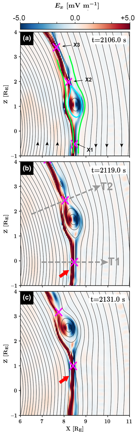
Figure 3. Three simulation timeframes (simulation box: 6 < X \text{ [RE]} < 11 and -1 < Z \text{ [RE]} < 4 at t = 2,106.0, 2,119.0 , and 2,131.0 s since the simulation initialization) to illustrate the temporal evolution of a magnetic island in the northern hemisphere magnetosheath. The color bar indicates E_x . The magenta “X” markers indicate the X-points, that is, saddle points in the magnetic flux function. The reconnecting field lines are shown in green. The newly formed magnetic island located between X1 and X2 is shown in cyan. The dashed lines in panel b provide two virtual spacecraft trajectories, T1 and T2.
