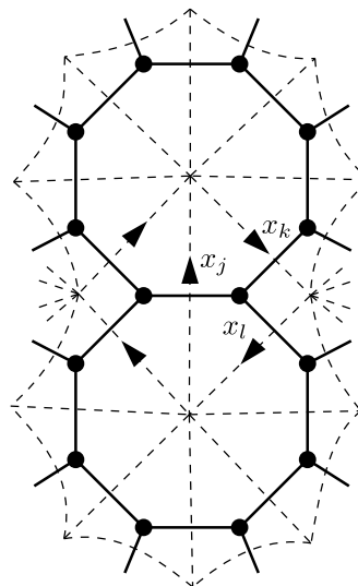
Figure 1: Tesselation with hyperbolic triangles whose angles are \frac{\pi}{4} .
