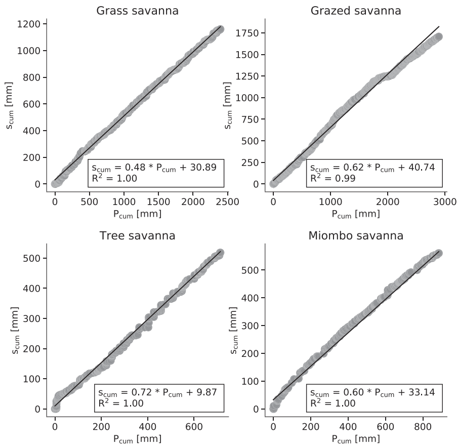
FIGURE 3 Relation between cumulative precipitation and cumulative positive increments in soil moisture for each site. The regression slope determined \gamma at 48%, 62%, 72% and 60% of the precipitation for the grass, grazed, tree and miombo savannas, respectively
