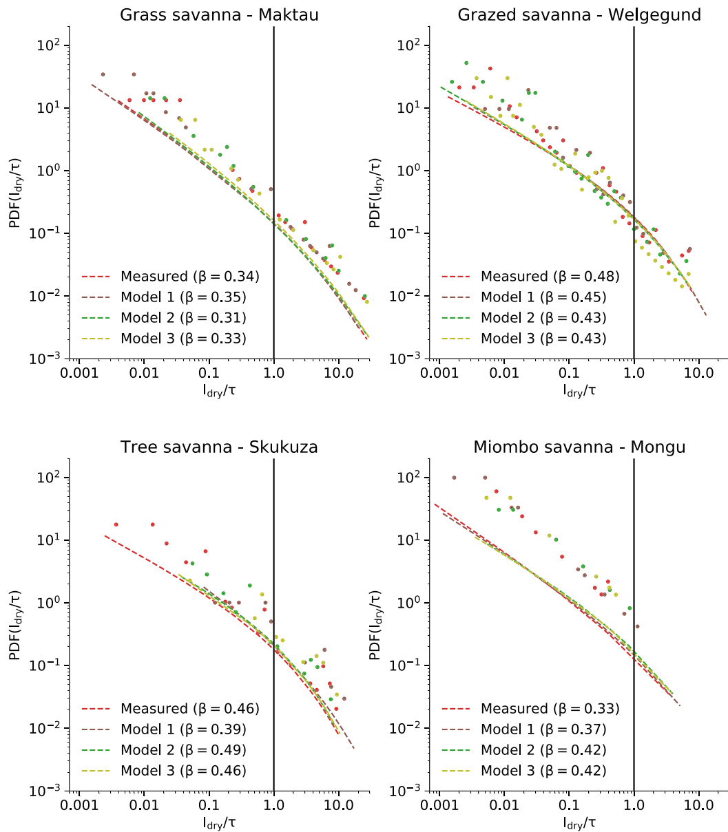
FIGURE 9 The probability density function (PDF) of persistence times of soil moisture below s^* divided by the site-specific memory timescale. The red, brown, green and yellow lines indicate the fit to the Equation 12 for the measured, Model 1, Model 2 and Model 3 results. The dots indicate logarithmically spaced bins. The vertical lines indicate the memory timescales determined at 21, 31, 17 and 50 days for the grass, grazed, tree and miombo savannas, respectively
