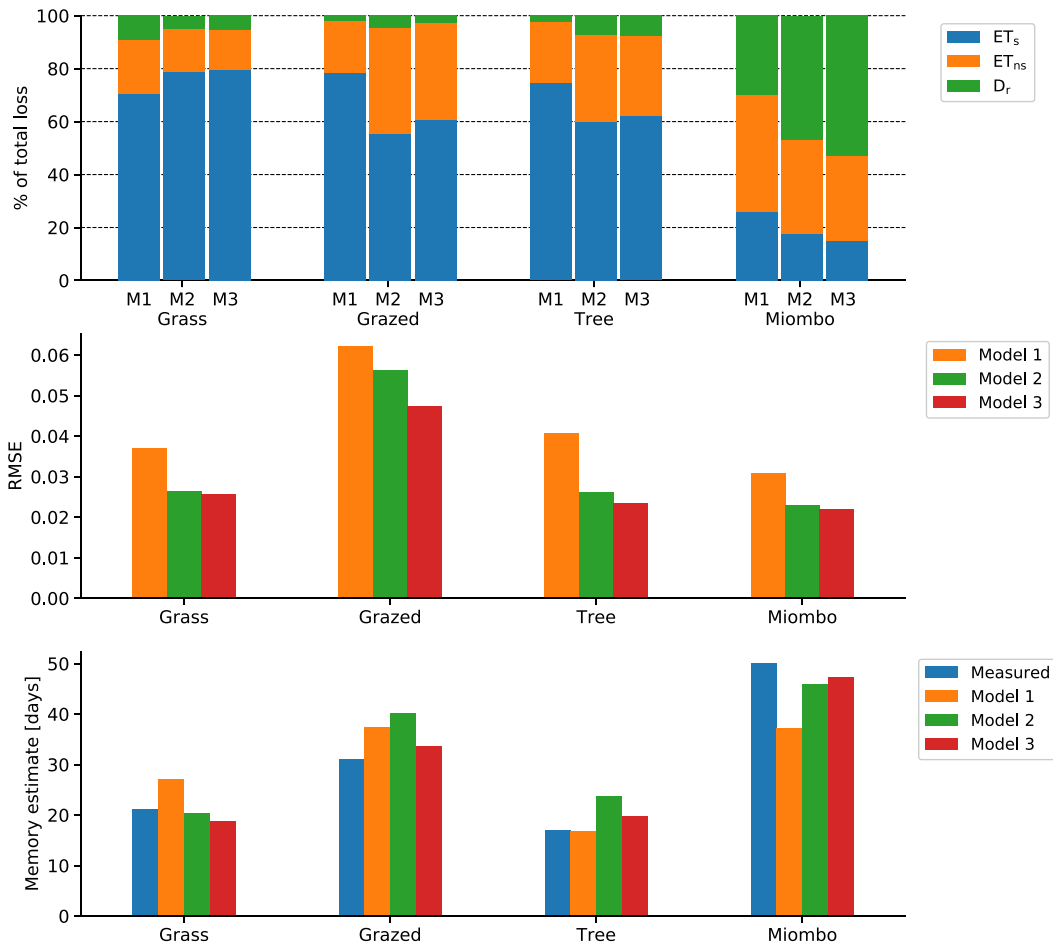
FIGURE 5 Comparison of water loss components, root-mean-square error (RMSE) and memory estimates. The total loss is partitioned to drainage ( D_r ), unstressed ET ( ET_{ns} ) and water stress ET ( ET_s )
