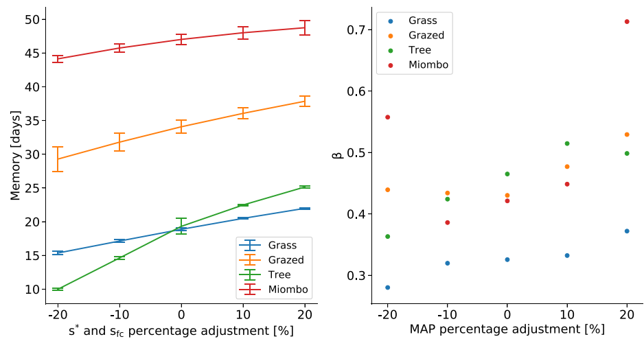
FIGURE 10 Model 3 memory sensitivity to changes in s^* and s_{fc} and Model 3 dry persistence parameter sensitivity to changes in mean annual precipitation (MAP). The error bars indicate \pm 1 standard deviation of the memory due to differences in MAP
