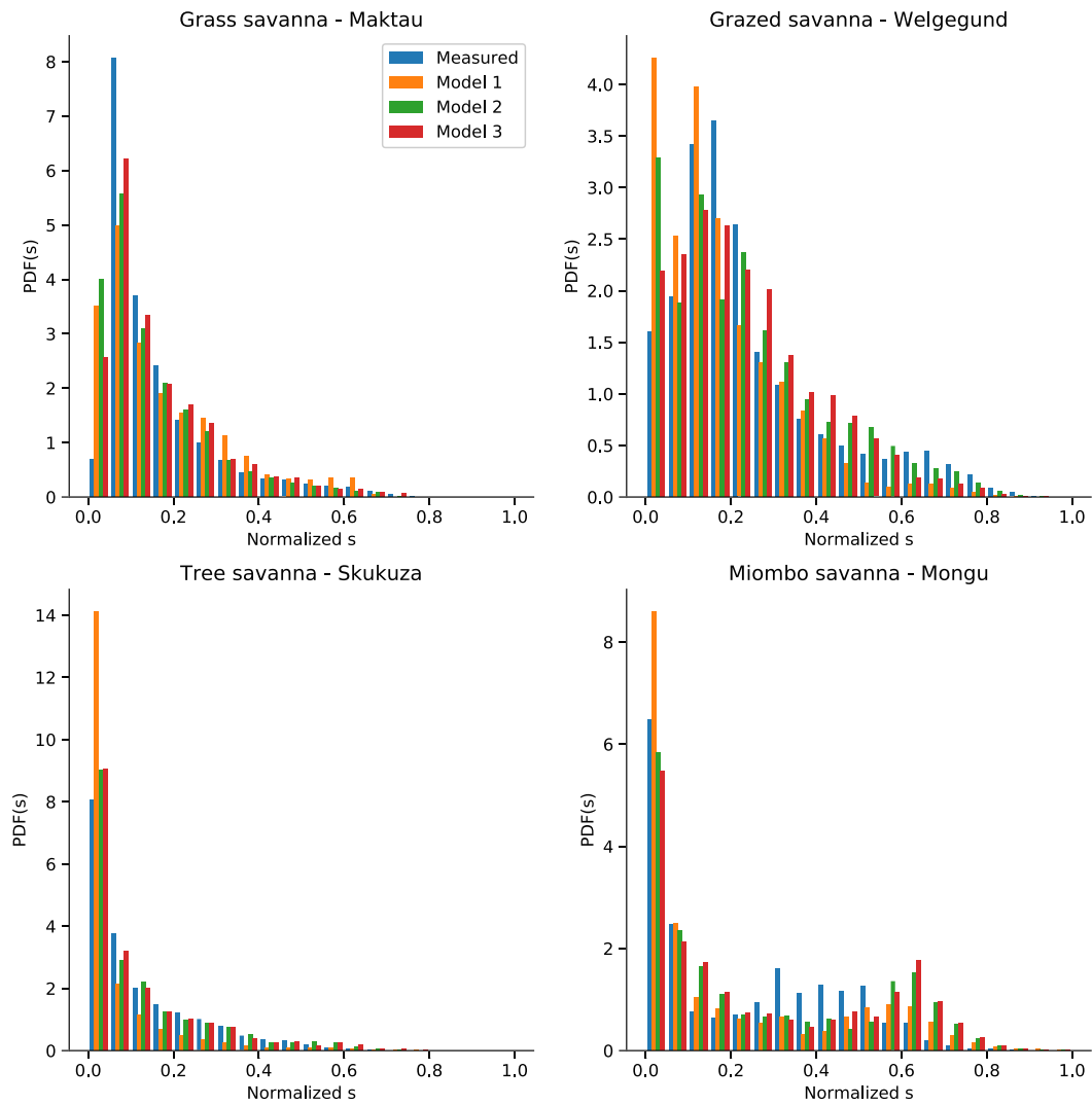
FIGURE 6 Histogram of normalized soil moisture for each savanna. The soil moisture values were rescaled to 0–1 range
