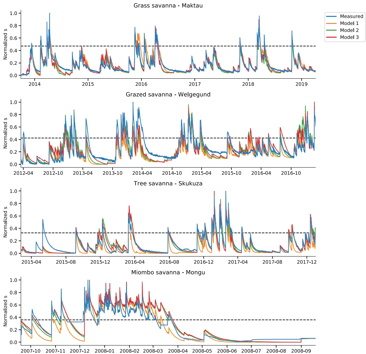
FIGURE 4 Time series of normalized soil moisture. The soil moisture values were rescaled to 0–1 range. The dashed line indicates the normalized value of the water-stress point ( s^* )
