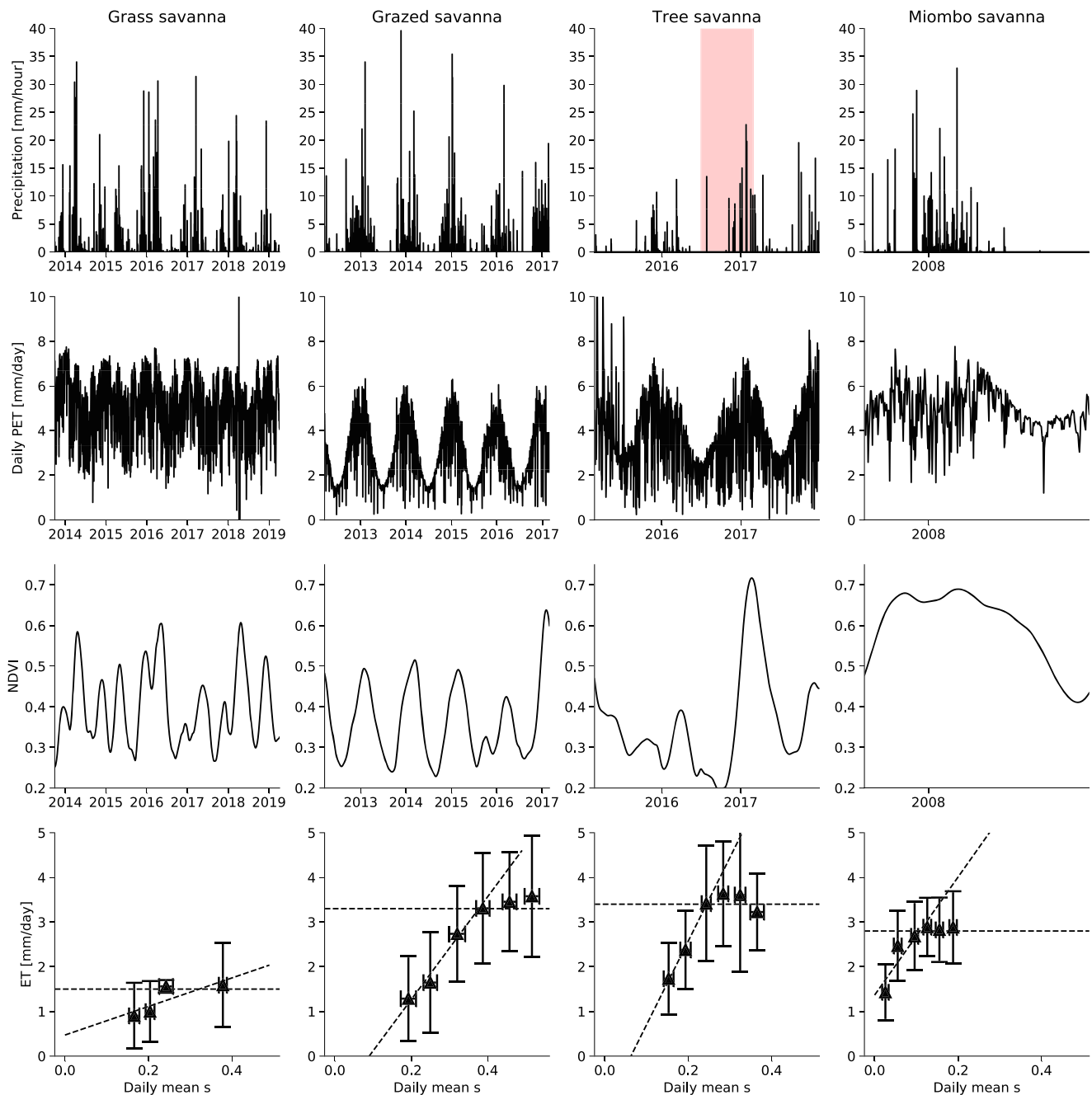
FIGURE 2 Time series of measured precipitation, potential evapotranspiration (PET) and normalized difference vegetation index (NDVI) at the grass, grazed, tree and miombo savannas. The red background indicates period of gapfilled precipitation at the tree savanna site. The last row shows the relation between measured daily mean soil moisture and eddy covariance-measured evapotranspiration. The rightmost bin of the linear increase in ET defines the plant water-stress threshold ( s^* ) and E_{max \times EC}
