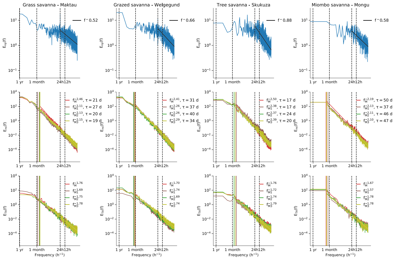
FIGURE 7 Normalized spectrum of measured precipitation ( E_{np}(f) ), measured and modelled soil moisture ( E_{ns}(f) ) and its telegraphic approximation ( ETA(f) ) for the four savanna sites. The red, brown, green and yellow colours show the measured, Model 1, Model 2 and Model 3 results, respectively. The memory timescales ( \tau ) are indicated with solid vertical lines with corresponding colour. The black dashed vertical lines indicate diurnal (12 h), daily (24 h), monthly and yearly time periods
