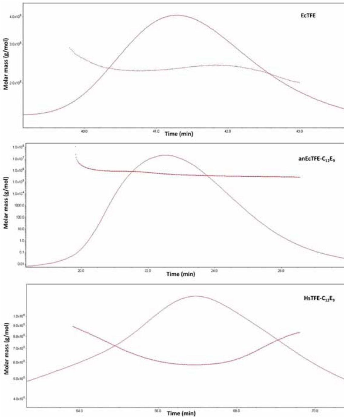
Supplementary Figure 4. The SEC-SLS analysis of EcTFE, anEcTFE (solubilized with C 12 E 9 detergent) and HsTFE (solubilized with C 12 E 9 detergent) using the Äkta Purifier equipped with a Superdex 200 10/300GL column (GE Healthcare), a Shodex refractive index detector and a Wyatt miniDAWN TREOS SLS detector. The plot of molar mass (horizontal red line) versus elution time is shown. Also shown is the corresponding SLS signal (curved red profile) showing the peaks of EcTFE, anEcTFE and HsTFE, eluting with an elution volume of 12.2 ml, 11.1 ml, and 10.9 ml respectively. The molecular mass of eluted EcTFE, anEcTFE and HsTFE is about 233 kDa, 535 kDa and 580 kDa respectively as calculated by the ASTRA Software.
