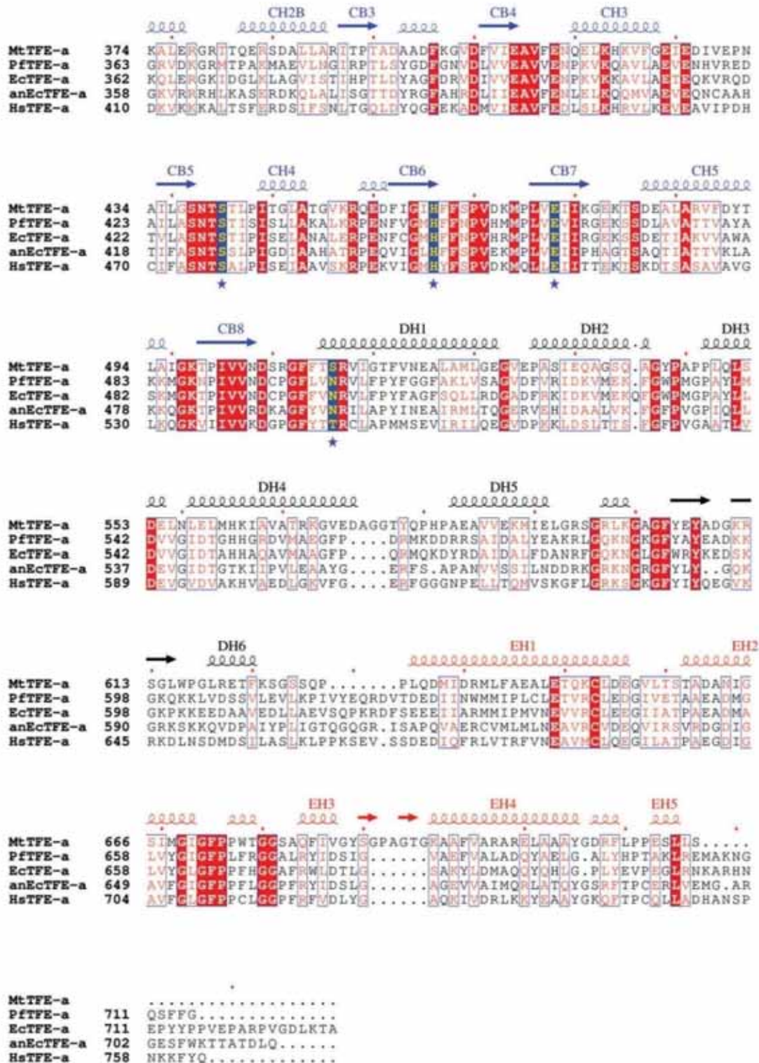
Supplementary Figure 1. Multiple sequence alignment of TFE- \alpha from different organisms. The secondary structure elements are from the structure of the \alpha chain of Mycobacterium tuberculosis TFE (identified as MtTFE-a) (PDB code: 4B3H). The active site residues in the hydratase and dehydrogenase domains are indicated with blue blocks with yellow residue names and blue stars at the bottom. The unique insertion in HsTFE- \alpha is identified with a red line below the sequence. Every tenth residue of anEcTFE- \alpha is marked with a red dot above the sequences.
