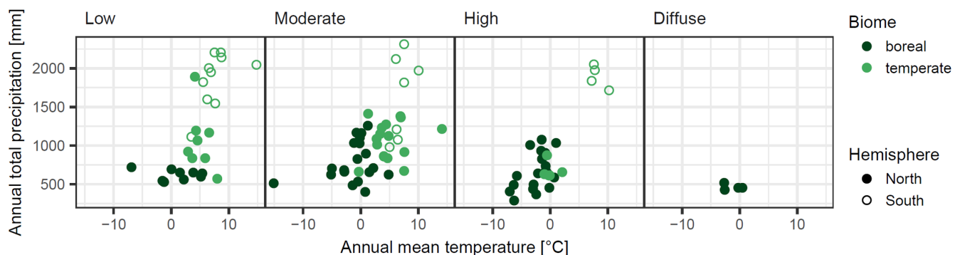
Figure 5. Location of the study landscapes in climate space for the four global clusters of disturbance activity.
