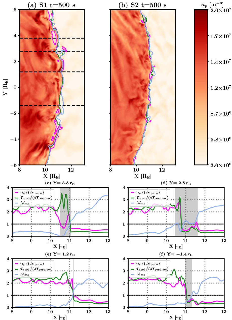
Figure 2. Proton number density overlaid with bow shock positions according to criteria for plasma density (fuchsia, n_p = 2n_{p,sw} ), solar wind core heating (green, T_{core} = 4T_{sw} ), and the magnetosonic Mach number (pale blue, M_{ms} = 1 ). Panel (a) is for S1 ( B_{sw} = 5 nT); panel (b) is for S2 ( B_{sw} = 10 nT). Both are at t = 500 s. Panels (c)–(f) show line profiles of the three bow shock criteria along the dashed black lines shown in (a), corresponding with differing amounts of shock non-locality.
