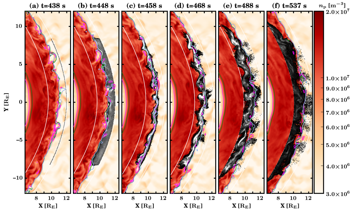
Figure 4. Test-particle propagation for simulation S1 and an Maxwellian 0.5 MK initialization at six different times. Vlasiator simulation proton number density is overlaid with the logarithmic density of test-particles in greyscale, with white indicating over 100 particles in a cell. Two black parabolas are the transmission boundary (left) and the injection boundary (right). Three contours indicate estimates of the local shock position: plasma compression (fuchsia, n_p > 2n_{p,sw} ), solar wind core heating (green, T_{core} > 4T_{sw} ), and the magnetosonic Mach number (pale blue, M_{ms} < 1 ).
