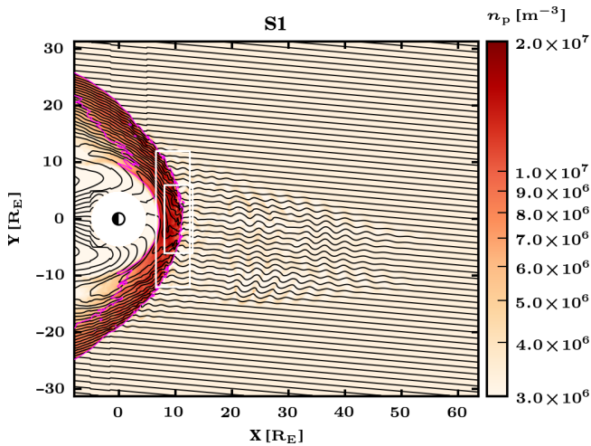
Figure 1. Overview of the Vlasiator simulation S1 ( B_{\text{IMF}} = 5 nT and M_A = 10 ) at time t = 500 s, with proton number density (colour map) overlaid with an estimate of the bow shock position according to plasma compression (fuchsia curve, n_p > 2n_{p,\text{sw}} ). Also shown are magnetic field lines (black curves) and two white overlapping rectangles indicating zoomed-in regions used for the analysis of local bow shock structure (smaller rectangle) and test-particle studies (larger rectangle).
