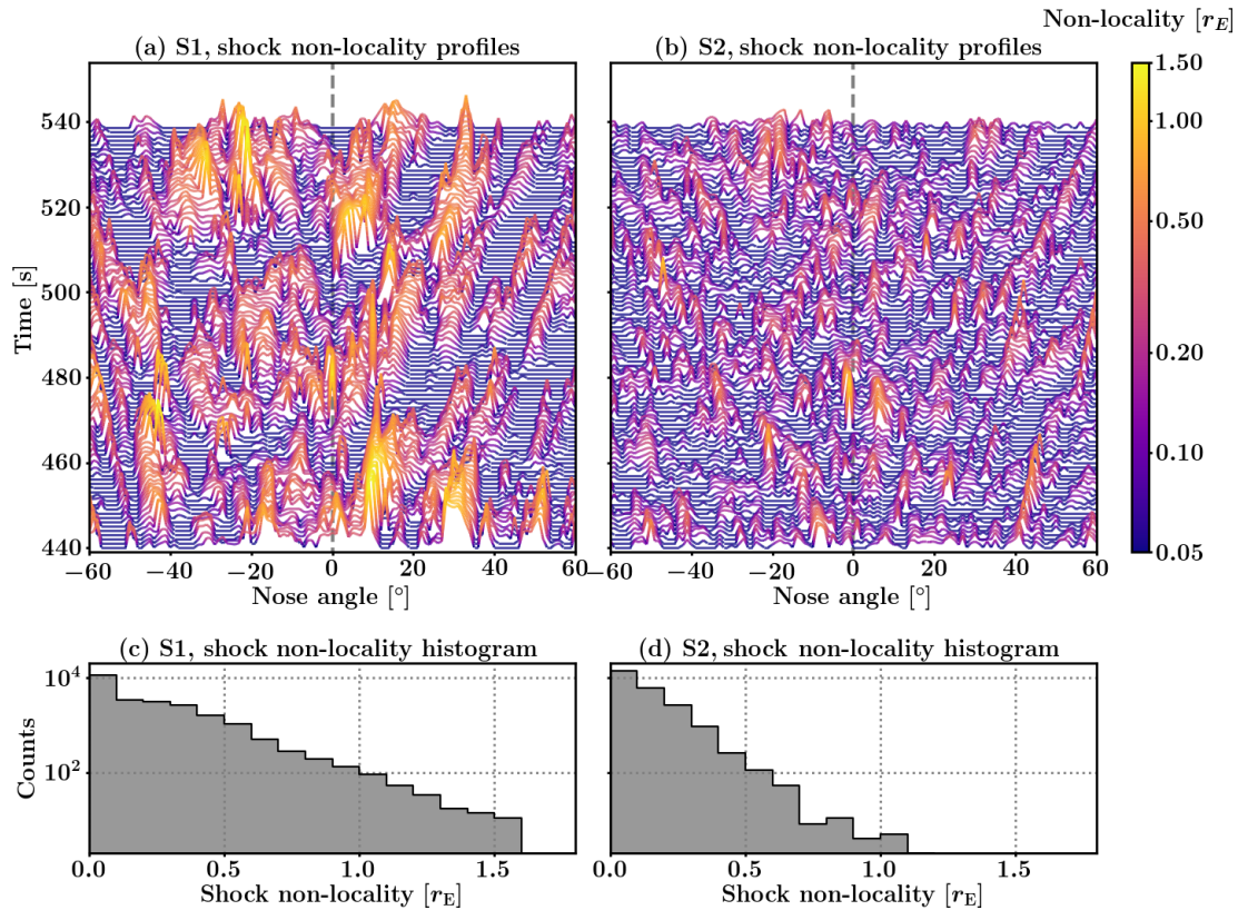
Figure 3. (a, b) Profiles of measured shock non-locality as a function of nose angle for simulations S1 and S2, respectively. The y axis indicates simulation time, used as the base level corresponding with a well-defined shock with a non-locality measure of 0. Regions of enhanced non-locality are shown as coloured peaks of the curve, as presented in the colour bar. A dashed vertical line indicates a nose angle of 0^\circ . Both panels show chains of enhanced non-locality regions which move away from the nose region and decrease in intensity as they approach the flanks. Under each stacked profile plot we show a histogram depicting the occurrence rate of different non-locality values, with (c) depicting S1 and (d) depicting S2.
