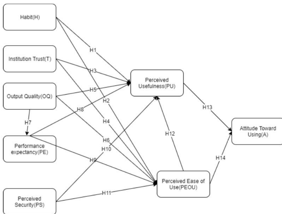
Figure 5 Research Model
