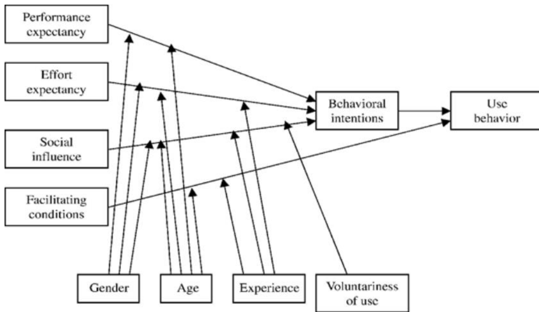
Figure 3. TUAUT model
