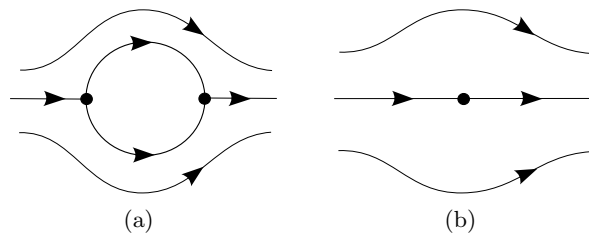
FIGURE 7. Here b > 1 and a \in (-1, 0) \cup (0, 1) . (a): Local phase portrait at r = 0 of system (18), (b): Local phase portrait at the origin of system (16).
