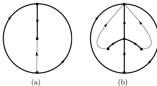
FIGURE 3. Global phase portrait of system (7) for b = 1 and a = 0 . (a): with c < 0 , (b): with c > 0 .
