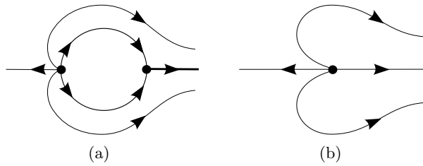
FIGURE 6. Here b > 1 and a \leq -1 (a): Local phase portrait at r = 0 of system (18), (b): Local phase portrait at the origin of system (16).
