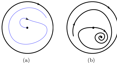
FIGURE 9. Global phase portraits of system (16) with b > 1 and a \neq 0 . (a): for |a| \geq 1 , (b): a \in (-1, 0) \cup (0, 1) .
