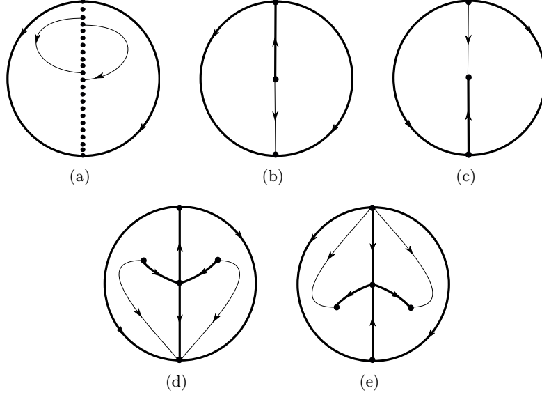
FIGURE 5. Global phase portrait of system (14) with a \neq 0 . (a): for c = 0 , (b): for c > 0 , (a - 1) \leq 0 , (c): for c < 0 , (a - 1) \geq 0 , (d): for c > 0 , (a - 1) > 0 , (e): for c < 0 , (a - 1) < 0 .
