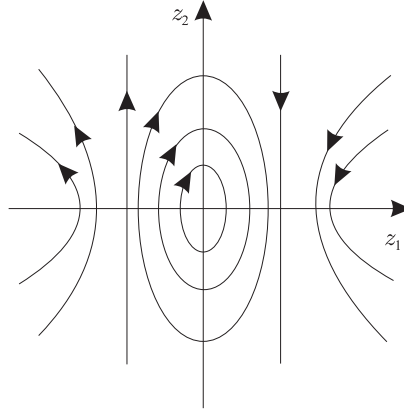
FIGURE 2. Phase portrait of system (3).
