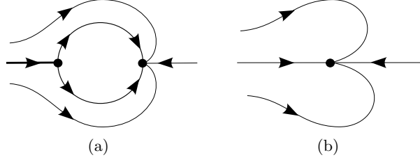
FIGURE 8. Here b > 1 and a \geq 1 . (a): Local phase portrait at r = 0 of system (18), (b): Local phase portrait at the origin of system (16).
