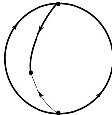
FIGURE 4. Global phase portrait of system (9).
