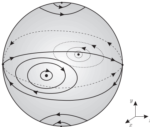
FIGURE 1. Phase portrait of system (1) on the sphere at infinity.
