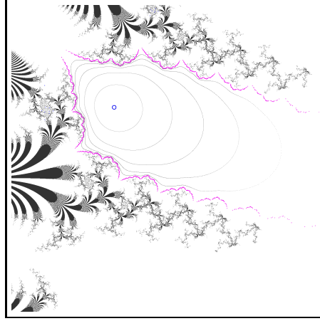
Figure 8: Point in a capture component for the critical value, so that the Siegel disk is conjectured to be unbounded. Details: a = (-0.33258, 0.10324) , upper left: (-1.5, 1.5) , lower right: (-3, -3) .
