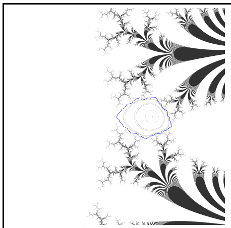
Figure 3: Julia set of the semi-standard map, corresponding to f_1(z) = \lambda z e^z . Upper left: (-3, 3) , lower right: (3, -3) . The boundary of the Siegel disk around 0 is shown, together with some of the invariant curves. The Fatou set consists exclusively of the Siegel disk and its pre-images.
