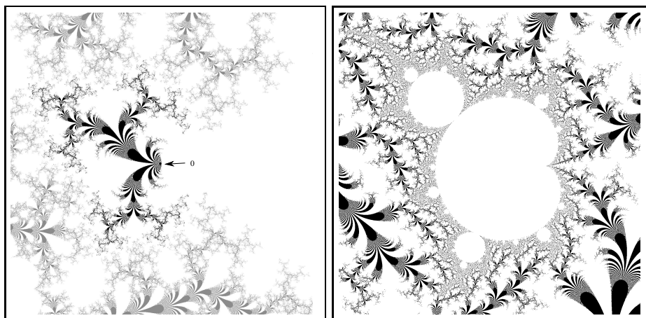
Figure 4: Left: “Crab”-like structure corresponding to escaping critical orbits (dark gray). Upper left: (-0.6, 0.6) , lower right: (0.6, -0.6) . In light gray we see parameters for which the orbit of v_a escapes. Right: Baby Mandelbrot set buried in the “crab like” structure. Upper left: (-0.336933, 0.1128) , lower right: (-0.322933, 0.08828) .
