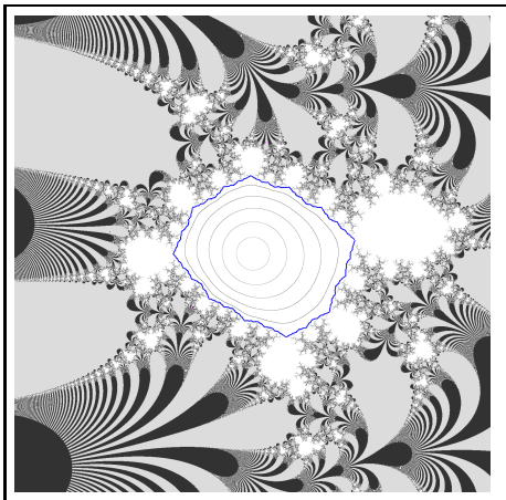
Figure 2: Julia set for a parameter in a semi-hyperbolic component (for the asymptotic value). Details: a = (-0.62099, 0.0100973) , upper left: (-4, 3) , lower right: (2, -3) . In light gray we see the attracting basin of the attracting cycle, and in white the Siegel disk and its preimages.
