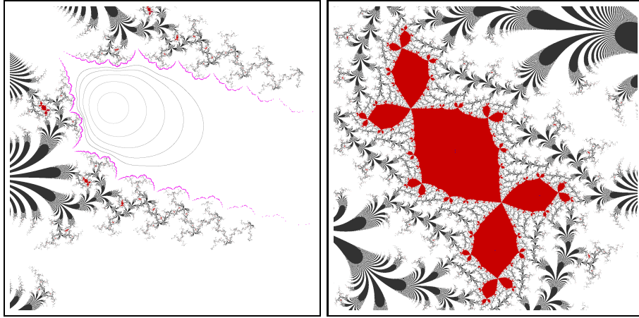
Figure 5: Left: Julia set for a parameter in a semi-hyperbolic component for the critical value. By Theorem 3.4 this Siegel disk is unbounded. Details: a = (-0.330897, 0.101867) , upper left: (-1.5, 1.5) , lower right: [3, -3] . Right: Close-up of a basin of attraction of the attracting periodic orbit. Upper left: (-1.1, 0.12) , lower right: (-0.85, -0.13) .
