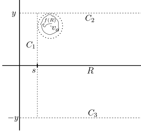
Figure 12: Sketch of the construction in Thm. 4.6 for the case \lambda_1, \lambda_2 > 0 .
