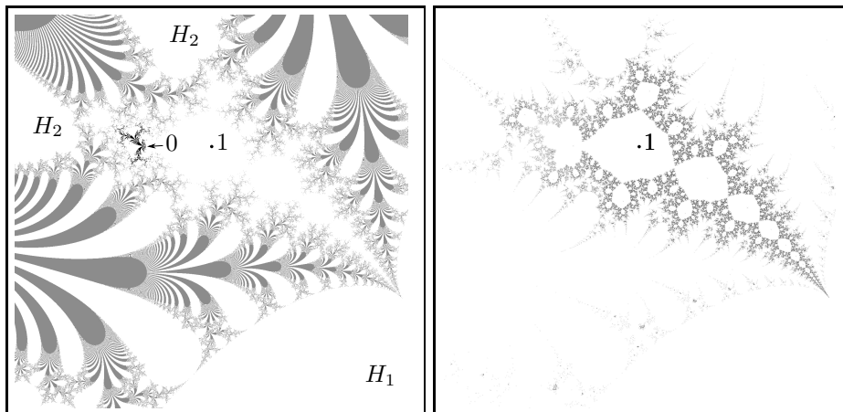
Figure 1: Left: Simple escape time plot of the parameter plane. Light grey: asymptotic orbit escapes, dark grey critical orbit escapes, white neither escapes. Regions labeled H_1 and H_2 correspond to parameters for which the asymptotic value is attracted to an attracting cycle. Right: The same plot, using a different algorithm which emphasizes the capture zones. Upper left: (-2, 2) , Lower right: (4, -4) .
