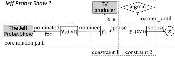
Figure 1: An example query graph for the question shown above. Assuming we start from the topic entity The Jeff Probst Show , the core relation path is the path linking The Jeff Probst Show to the lambda variable x . There are two constraints in the query graph. Note that y_1 and y_3 are CVT nodes used for n -ary relations.
