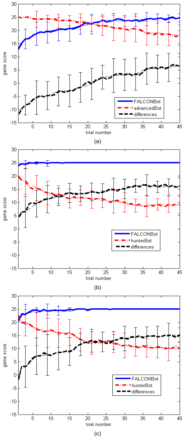
Fig. 10. Game scores of FALCONBot playing against different bots in different maps. (a) VS. advancedBot in the Spirit map. (b) VS. hunterBot in the Idoma map. (c) VS. hunterBot in the Spirit map.
