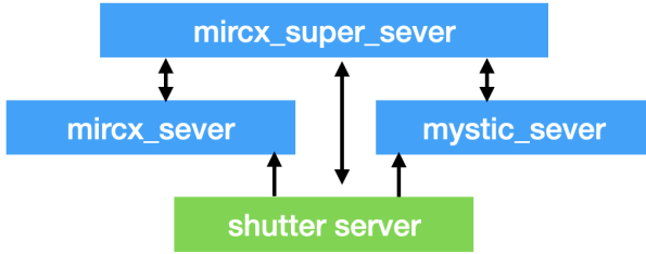
Figure 12. Observing coordination of MIRC-X and MYSTIC instruments. mircx_super_sever server coordinates the data taking process for the MIRC-X and MYSTIC instruments. For example, it opens the CHARA shutters and starts the integration on both instruments.
