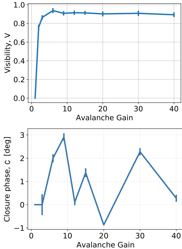
Figure 19. Visibility (top) and closure phase (bottom) averaged across all wavelength channels (prism R = 50 ) measured using the internal light source while varying the detector avalanche gain. The visibility variation is less than 2%, and closure phase variation is less than 3^\circ . The bottom plot data is very noisy because of a lack of good flat fielding reference for each avalanche gain.
