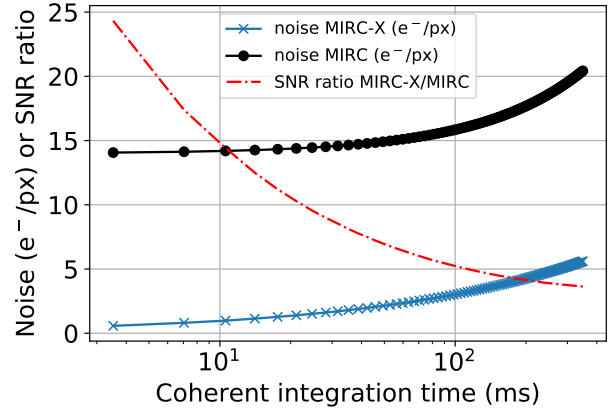
Figure 18. Total noise model for MIRC-X camera at gain 40 (readout noise of N_{\text{RON}} \approx 0.5e^-/\text{px} RMS and background of \approx 90e^-/\text{px} \cdot \text{s}^{-1} ) and for the MIRC camera (readout noise of N_{\text{RON}} \approx 14e^-/\text{px} RMS and background of \approx 340e^-/\text{px} \cdot \text{s}^{-1} ). The MIRC-X camera delivers 14.5 (5.5) better SNR than MIRC for 10 ms (100 ms) coherent exposures.
