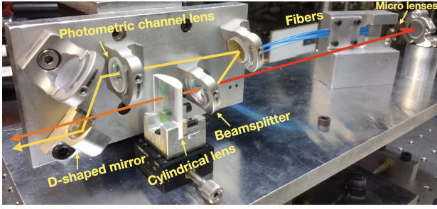
Figure 3. Front view of the MIRC-X beam combiner.
