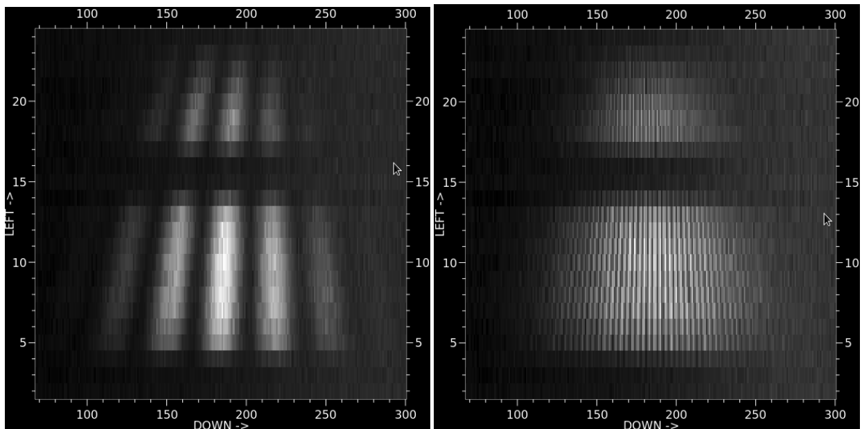
Figure 16. Fringes in J+H band fringes observed for beam pairs 1 & 2 (smallest spatial frequency) and 1 & 6 (highest spatial frequency) using the internal light source. The horizontal axis and vertical axis are the spatial and spectral directions, respectively, in detector pixel coordinates. The dark patch in between the J and H-band fringes is due to the notch narrow-band filter used to filter out the CHARA metrology laser.
