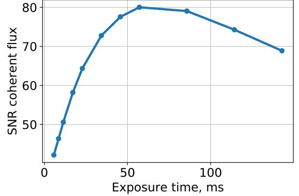
Figure 20. Wavelength-averaged SNR of the coherent flux as a function of coherent integration time for UT 2019-08-27. The SNR of the coherent flux increases with coherent integration time until it equals the atmospheric coherence time of \tau_0 \approx 60 ms.
