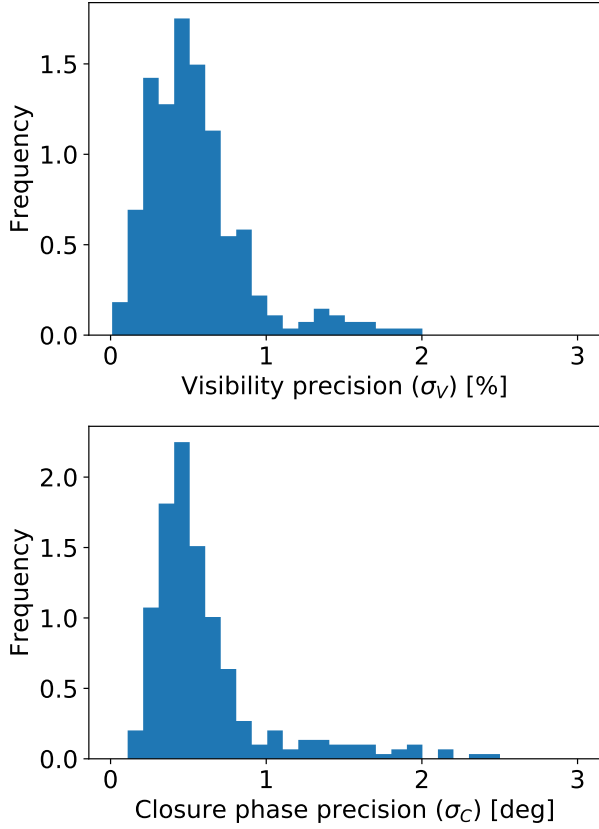
Figure 22. Histogram of the wavelength-averaged visibility (top) and closure phase (bottom) precision estimated from on-sky observation of bright calibrators on UT 2019-09-04. The precision is the statistical 1\text{-}\sigma uncertainty estimated by the pipeline.
