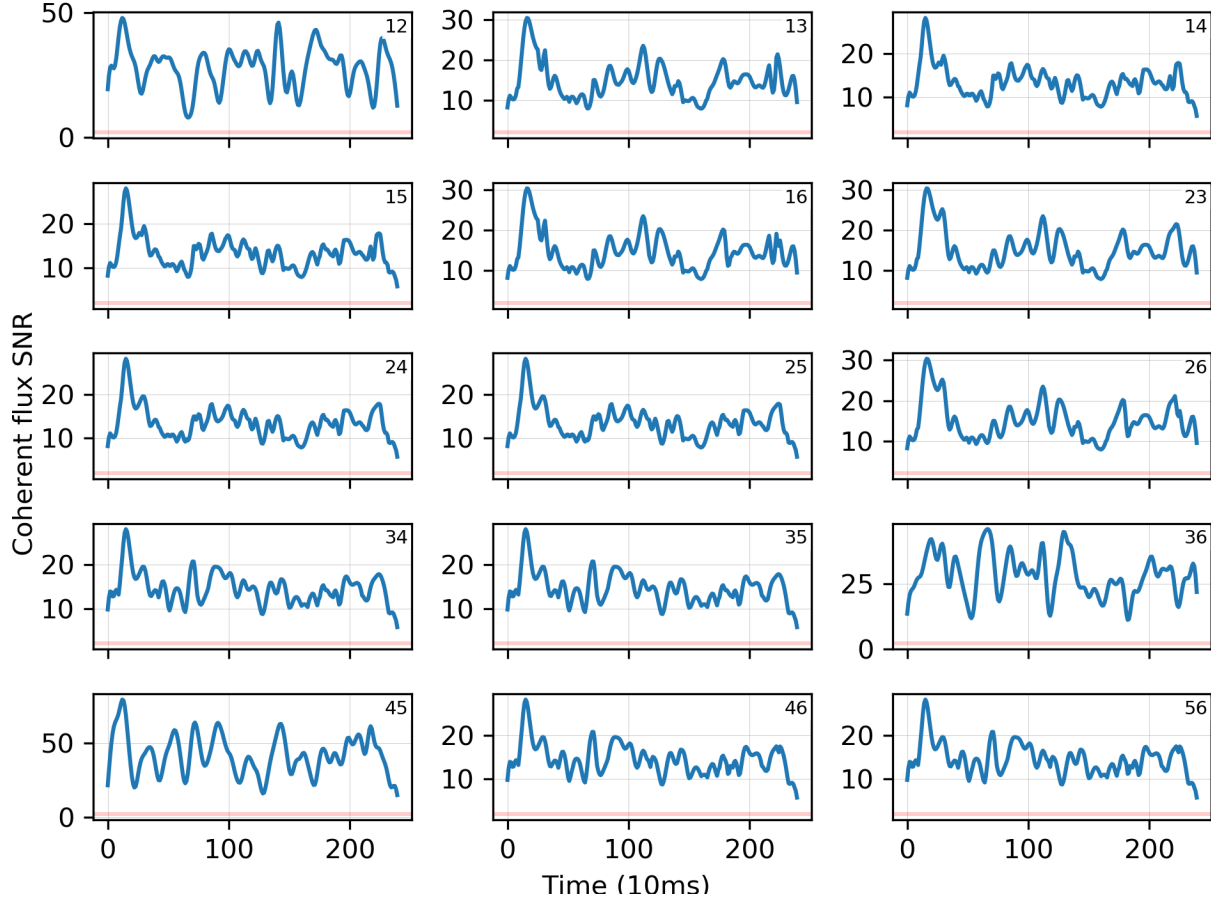
Figure 21. SNR of fringes recorded on a faint YSO, GW Ori, m_H = 7.1 on UT 2019-08-27 under exceptional seeing conditions ( r_0 \approx 11 cm, wind speed \approx 2.7 m/s). The red color is the SNR threshold above which fringes are considered. The 15 panels are for the 15 baselines. The baseline pair numbers are indicated in each panel. The data are reduced with a coherent integration time of 30 ms.
