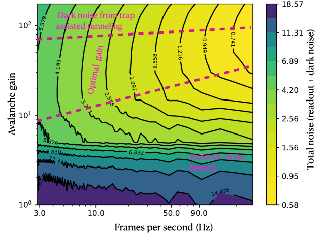
Figure 8. Total noise ( e^- ), the sum of readout noise + dark noise, as a function of the avalanche gain and frame rate. The axes are in a log scale. At gain values below 10, the performance of the detector is readout-noise limited. The optimal gains as a function of frame rate are shown in the gap between two dashed lines. At gain values above 60, trap assisted tunneling defects come into place and add additional dark noise.
