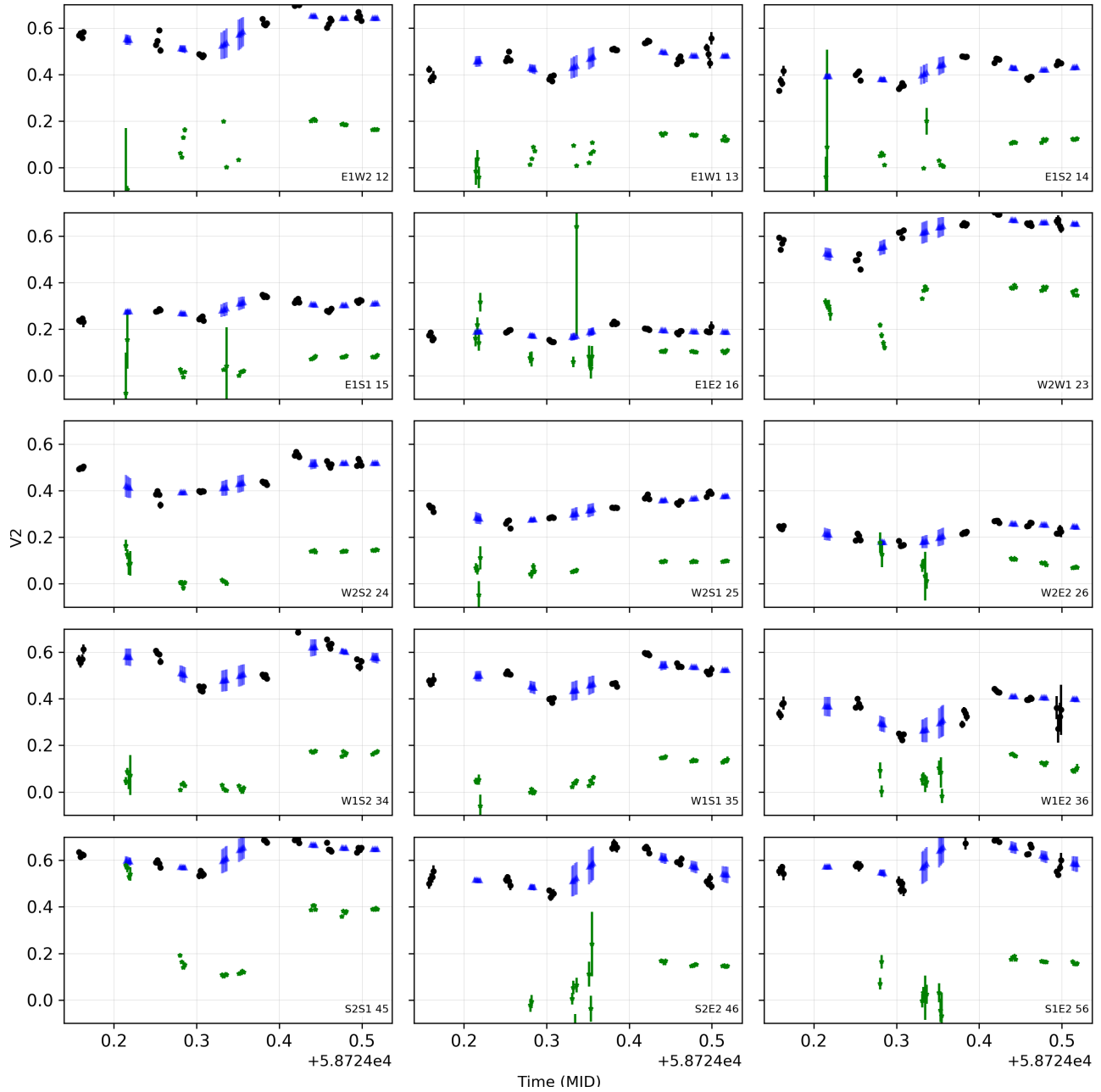
Figure 23. Transfer function squared visibility measurements for MIRC-X observed on UT 2019-08-29. The black color represents the transfer function estimates for calibration stars. The blue color represents the interpolation of the transfer function at the time of science-star observations. The green color represents the observations of scientific objects. The observed calibrators are HD 199580 (0.50 mas), HD 228852 (0.53 mas), HD 204050 (0.42 mas), HD 21820 (0.47 mas), HD 28855 (0.30 mas) from left to right and with H-band angular diameters in parentheses (JSDC; Bourges et al. 2017). The majority of the visibility variation seen in the calibrators is due to variations in the system visibility due to seeing and different pointings on the sky (polarization changes).
