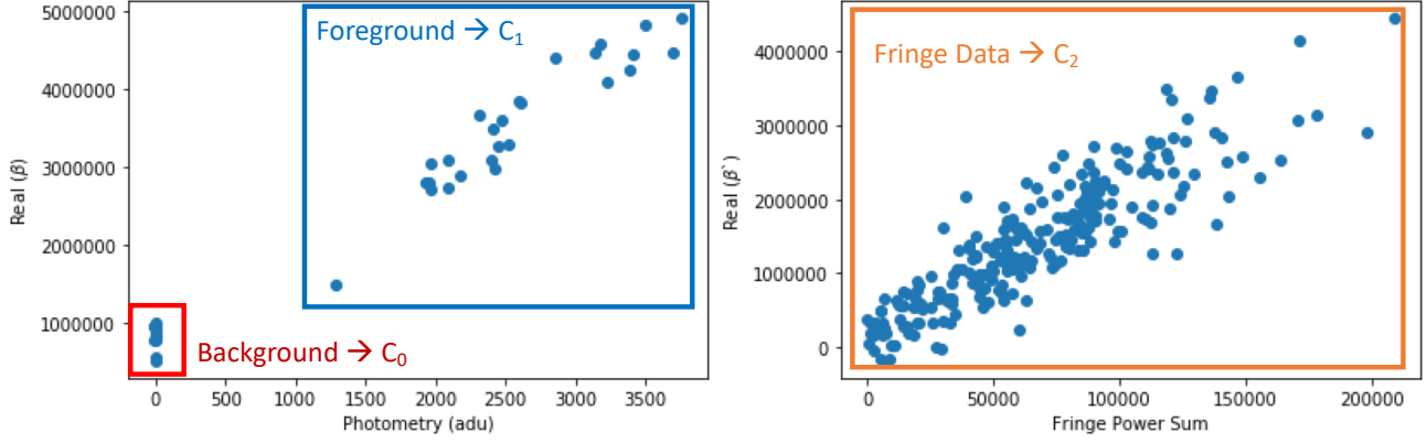
Figure 27. Left panel: real part of the bispectrum for all BACKGROUND and FOREGROUND files of the night to compute the bispectrum bias coefficients C_0 and C_1 from equation B1. Right panel: measurement of \beta' = \beta - C_0 - C_1 N in the DATA files of the same night, to show the relationship for the C_2 term. We compute these coefficients for each spectral channel, and perform a least-squares fit of the entire dataset to measure the coefficients.
