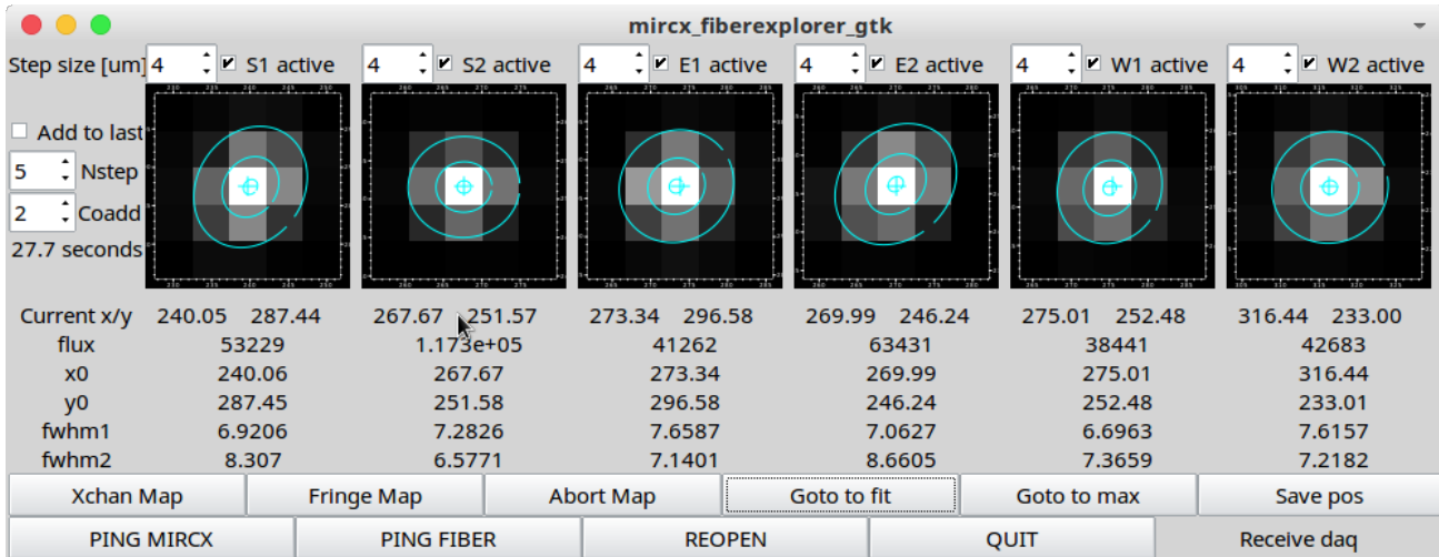
Figure 14. mircx_fiberexplorer_gtk interface. The flux injection into the fiber is optimized by scanning the fiber in X and Y directions. The resulting map is fitted with a Gaussian model to find the position that results in the best flux injection. The GUI shows the Gaussian fit centers (location of fiber motors where the maximum flux can be found), flux, and FWHM. Xchan Map performs a fiber explorer map by searching for the flux using the six photometric channels simultaneously. Fringe Map performs a search using the flux in the fringe window and searches for the flux in one beam at a time.
