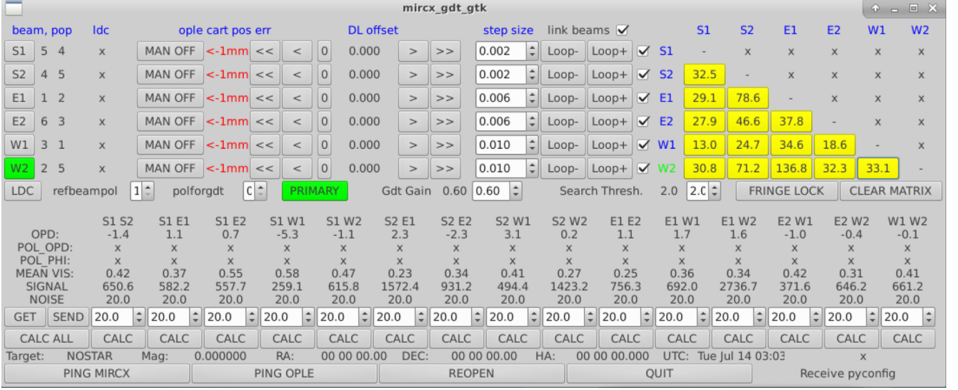
Figure 26. mirrcx_gdt_gtk , the MIRC-X group delay tracking GUI. The CALC ALL button measures the thresholds of fringe detection by moving the carts away from fringes. LOOP+ and LOOP- buttons enable the fringe search with step sizes entered adjacent to these buttons. Once the fringes are found on a particular pair of baselines, the buttons in the matrix are colored, and these fringes can be locked by pressing the FRINGE LOCK button. The PRIMARY button allows switching between the CHARA delay lines and the internal delay lines when sending the OPD offsets for correction. The wavelength dispersion correction is activated with LDC button. The GUI shows the status of beams, pops, and cart position error. It also shows the group delay measurement parameters OPD, SNR in the measurement, polarization OPD, wavelength-averaged visibility, etc.
