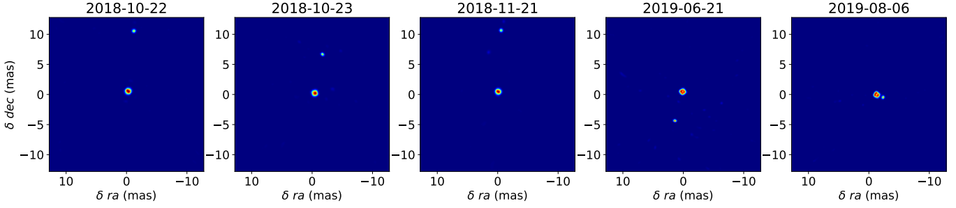
Figure 24. Model-independent image reconstruction of \iota Peg at several epochs using the squeeze software. Observations of each night are reduced independently, and images are reconstructed. North is up and East to the left. The image maximum is normalized to unity, and the color scale is linear. The primary star is centered in the image window.
