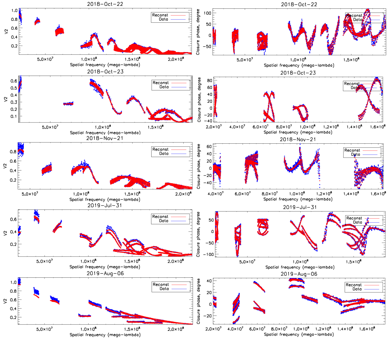
Figure 29. The squared visibility V^2 and closure phase C of \iota Peg for different epochs. The blue and red curves are the data and fitting of image reconstruction. V^2 is a measure of spatial resolution of the source by a given baseline at a given wavelength. The closure phases are related to the asymmetry of the binary system: the closure phase is null for a centro-symmetric target.
