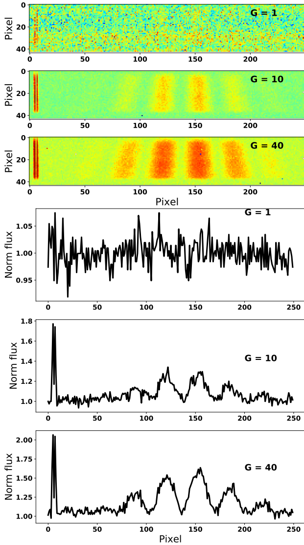
Figure 17. MIRC-X two-beam fringes obtained with the internal source at avalanche gain 1, 10, and 40. The top three panels are the 2D images. The bottom three panels are for one spectral channel. Flux is normalized with respect to maximum flux in gain 1. In each panel, left are the photometric channels, and right are the fringes. For the avalanche gains above 10, the detector is in the sub-electron readout noise regime. For comparison, the MIRC-X performance at gain = 1 is approximately equal to the performance of MIRC’s PICNIC detector. The photometric channels appear close but they are separated by 3 pixels peak-to-peak with beam size of \sim 0.6 pixel in FWHM.
