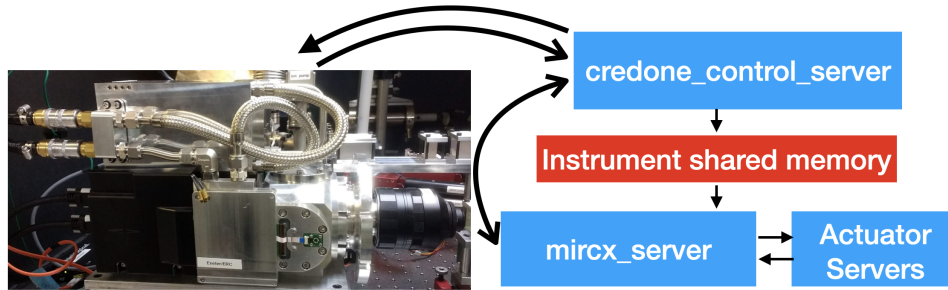
Figure 11. Architecture of MIRC-X data acquisition. The C-RED ONE camera images are grabbed in the MIRC-X computer and written in a shared memory by the credone_control_server . The mircx_server reads the shared memory and implements image processing, fringe tracking, and data recording to an solid state drive. The mircx_server uses a standard client/server model to monitor and update the C-RED ONE configuration and to talk to actuators.
