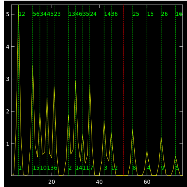
Figure 13. Real-time display of power spectrum of MIRC-X fringes. The mircx_rtd_gtk GUI displays the power spectrum peaks at the expected frequencies (vertical dashed green lines) for the 15 pairs of beams. The red line represents the background noise pixels considered in the estimation of power spectrum peaks. The green numbers represent the beam pair (top) and the baseline number (bottom). The arrangement of beam pair 1 and 2 being the lowest spatial frequency and 1 and 6 being the highest spatial frequency (see the design in Figure 6). The unequal fluxes of beams degrade the contrast of raw fringes. The fringe contrast is low for highest frequency fringes in a comparison because of pixel under-sampling and uncorrected camera vibrations, which affect the under-sampled fringes the most.
