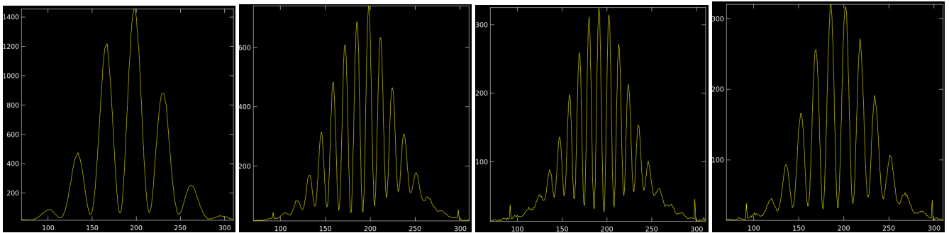
Figure 15. Contrast of H-band fringes observed for nearest beam pairs 12, 34, 45, and 56 using the internal light source. A single spectral channel line is presented. The non-calibrated visibility contrasts for the nearest pairs are 85 to 95%. The X-axis is the spatial frequency direction in pixels. Y-axis is flux in ADU. The different beam pairs have different spatial frequencies because the separation between the two beams in each pair is non-redundant.
