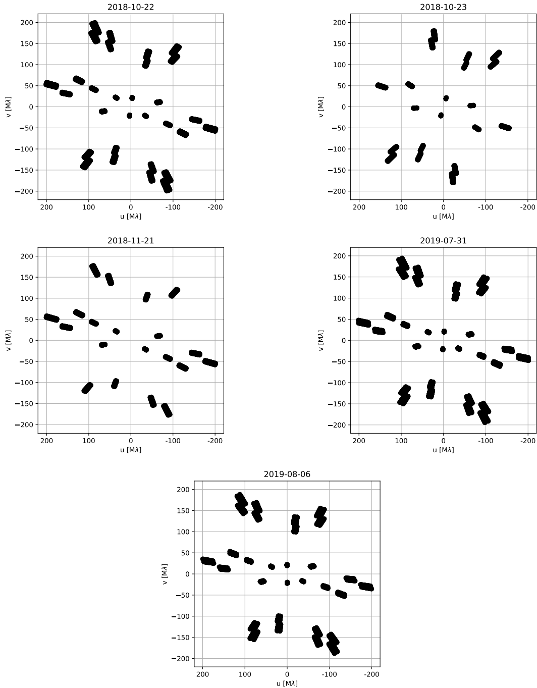
Figure 28. (u, v) -coverage of observations of object \iota Peg are shown. Each panel corresponds to an epoch. The radial tracks represent spectral dispersion over 34 spectral channels observed with grism R = 190 .
