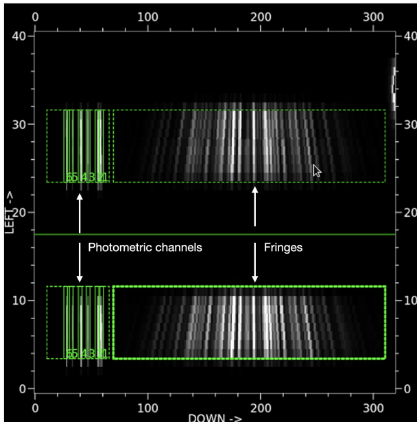
Figure 5. H-band photometric channels and fringes (see Section 3.6) obtained with a Wollaston prism. The upper and lower panel present fringes and photometric channels in the orthogonal polarizations (horizontal/vertical). The green numbers are the numbers of photometric channels.
