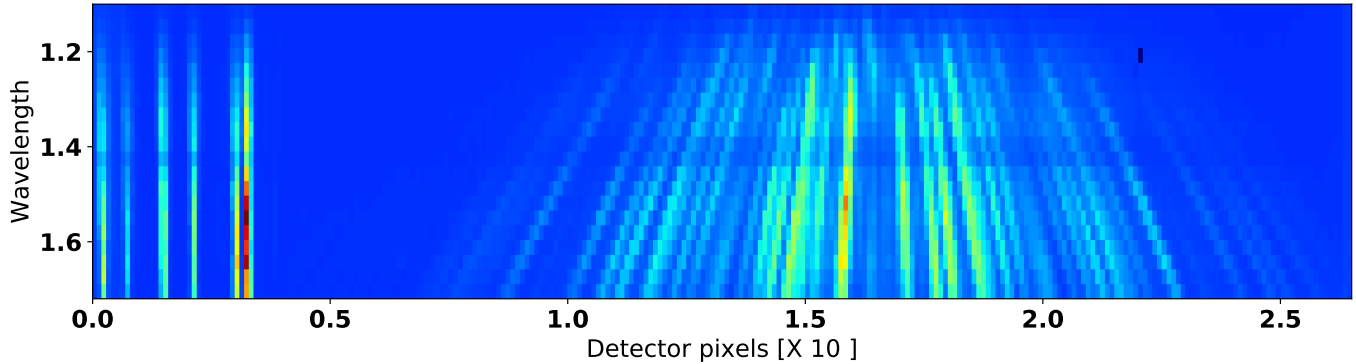
Figure 7. Six beam J+H band images recorded with the internal light source (STS). The spatial direction is horizontal and the spectral direction is vertical. Wavelength is in \mu\text{m} . The photometric channels on the left are the images of the cores of the non-redundant fibers in the V-groove. The photometric channels of beam 2 and 1 (right-most) are the closest one to each other, but are separated by more than one pixel. The fringe pattern (right) encodes the coherence of the 15 pairs at different spatial frequencies. This image is with the R = 50 prism and no Wollaston. The Wollaston creates two of such images separated in the vertical direction, one for each polarization.
