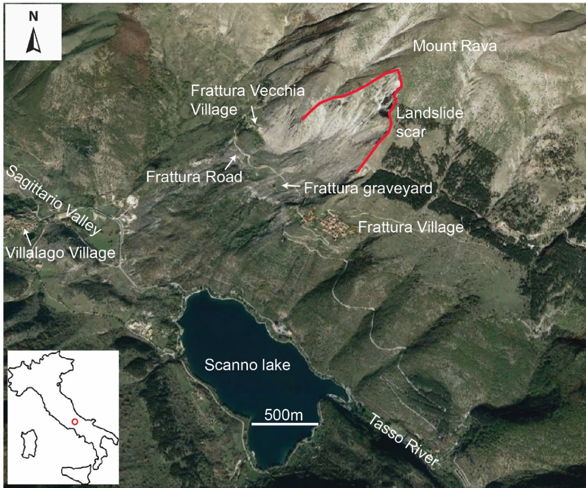
Figure 1. SW flank of the Mount Rava with the Scanno landslide and landslide scar (in red) highlighted. Location of the study area is shown in the inset.
