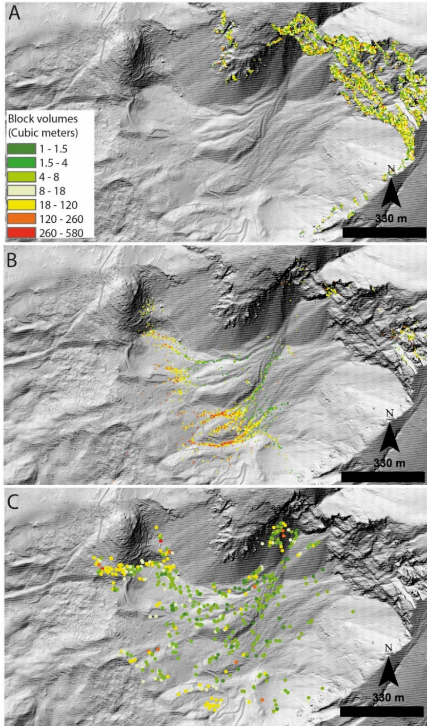
Figure 18. (A) Example of block volume distribution within release cells using the proposed procedure. (B) Results of the rockfall simulations using relative rockfall block volume frequency. (C) Map of recent rockfall events. Color scheme reported in (A) is the same used for (B) and (C).
