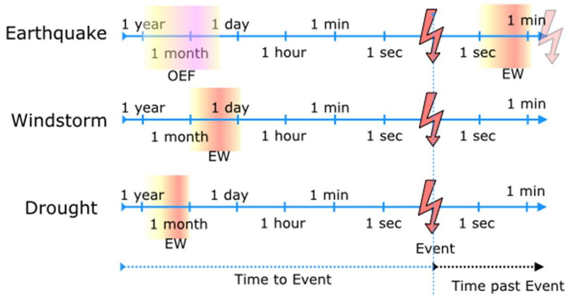
Figure 2: The concept of early warning (EW) and its placement in time with respect to the actual occurrence of the event, exemplified for earthquakes, windstorms and droughts. In the case of earthquakes, even very short lead times, up to 60 seconds after the occurrence of the event (dark flash), still allow to automatically trigger real-time mitigation measures, such as emergency braking of high-speed trains, before the most potentially dangerous earthquake waves reach a given location (light flash). For earthquakes also Operational Earthquake Forecasting (OEF) is indicated. Windstorms can be forecasted with lead times from a couple of hours to several days. The lead times of droughts are even longer, in the range of one to several months.
