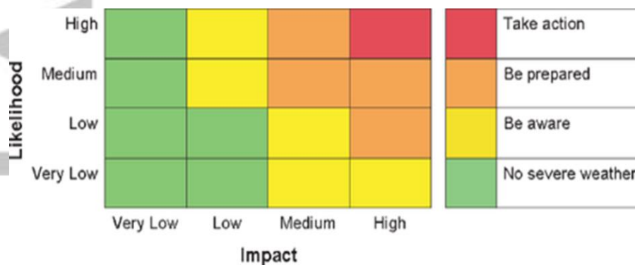
Figure 4: Weather impact matrix and color key for the UK National Severe Weather Warning Service (from Neal et al., 2014). Green signifies weather with no significant impact on peoples’ day-to-day activities. Yellow signifies ‘be aware’ and stay up to date with the latest forecast, amber signifies ‘be prepared’ to take action. Red signals ‘take action’ to mitigate impacts.
