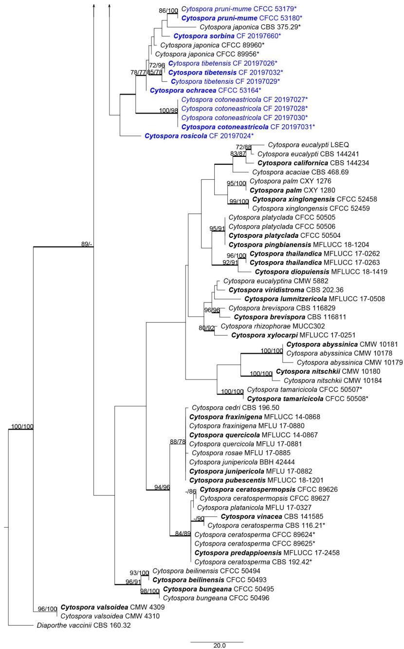
Figure S1. Phylogram of Cytospora based on ITS gene. MP and ML bootstrap support values above 70 % are shown at the first and second position. Thickened branches represent posterior probabilities above 0.95 from BI. Ex-type strains are in bold. Strains in current study are in blue. All the Cytospora species listed from Rosaceae plants in China are marked with *.
