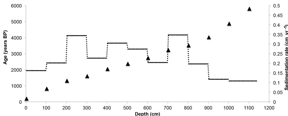
Figure 3. Age–depth model of core MSM45-31-1. Black triangles mark the calibrated ages of the AMS radiocarbon dates. The black dotted line marks the sedimentation rate ( \text{cm yr}^{-1} ).
