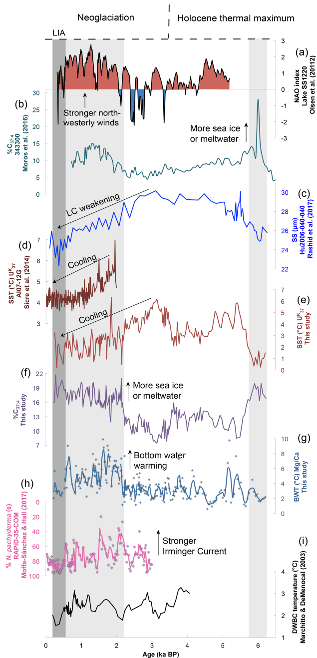
Figure 6. (a) The NAO index (Olsen et al., 2012) with positive (red) and negative (blue) phases. (b) \%C_{37:4} in core 343300 (Moros et al., 2016). (c) Sortable silt mean ( \mu\text{m} ) in core Hu2006-040-040 (Rashid et al., 2017). (d) SST record in Newfoundland core AI07-12G (Sicre et al., 2014). (e) SST record based on the U_{37}^K index (this study). (f) Higher levels of \%C_{37:4} are interpreted as reflecting a longer sea ice season or meltwater. (g) BWT estimates are based on Mg/Ca ratios in benthic foraminifera N. labradorica and reflect subsurface conditions. (h) Lower abundances of polar water planktic foraminifera species N. pachyderma sinistral in central Labrador Sea core RAPiD-35-COM indicate warming due to stronger IC inflow (Moffa-Sánchez and Hall, 2017). (i) Mg/Ca temperature estimates representing the Deep Western Boundary Current (Marchitto and deMenocal, 2003). Grey vertical bars highlight periods of pronounced oceanographic change.
