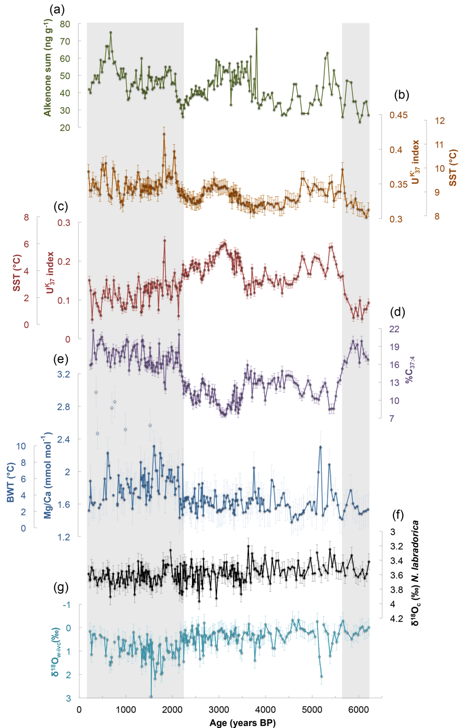
Figure 4. Down-core record of MSM45-31-1 showing (a) alkenone sum, (b) U_{37}^{K'} index displayed with 0.01 uncertainty, and respective SST estimates, (c) U_{37}^K index displayed with 0.01 uncertainty and respective SST estimates, (d) \%C_{37:4} displayed with 0.8% uncertainty, (e) Mg/Ca ( \text{mmol mol}^{-1} ) of N. labradorica displayed with 0.19 \text{mmol mol}^{-1} uncertainty and respective BWT estimates, (f) \delta^{18}\text{O}_{\text{calcite}} (‰-V-PDB) of N. labradorica displayed with 0.11‰ uncertainty, and (g) \delta^{18}\text{O}_{\text{w-ivc}} (‰-V-SMOW) displayed with 0.35‰ uncertainty. Grey vertical bars highlight periods of pronounced oceanographic change.
