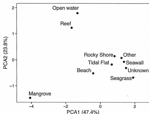
Fig. 1. Principal component analysis of the Tier 1 indicators of scientific value.
