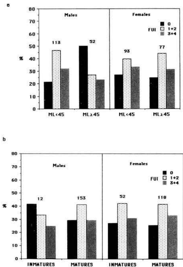
FIG. 2. — Percentage of stomachs with different Fullness Index (FUI) for each sex and size group (a) and sex and maturity state (b) of Sepia elegans . Number of specimens is given above histograms. ML: mantle length in mm.
