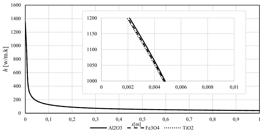
Figure 18. Comparison of average heat transfer along the plate for water based nanofluids with different nanoparticles ( \phi = 0.04 )
