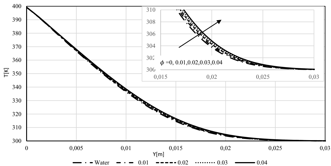
Figure 14. The temperature profiles for different value of \phi , ( Al_2O_3 -water)
