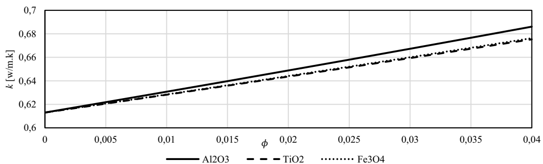
Figure 5. The effect of nanoparticles on the thermal conductivity
