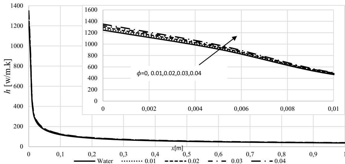
Figure 17. The average heat transfer along the plate ( \text{Al}_2\text{O}_3 -water case)
