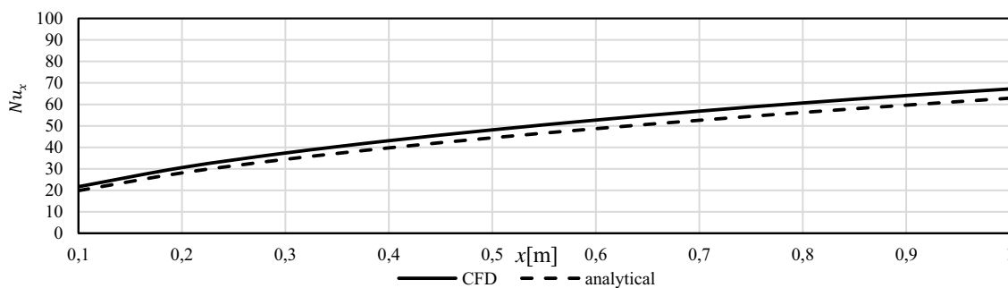
Figure 8. The local Nusselt numbers' comparison for water
