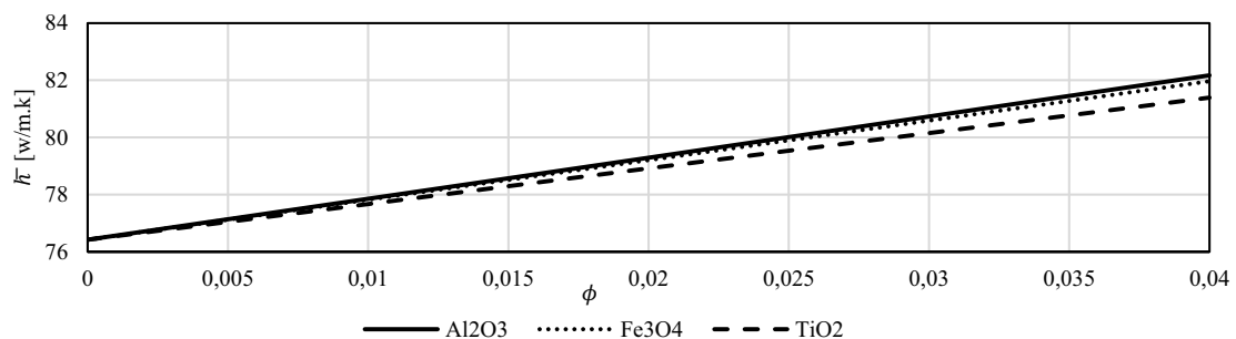
Figure 16. The effect of adding nanoparticles on the average heat transfer coefficient
