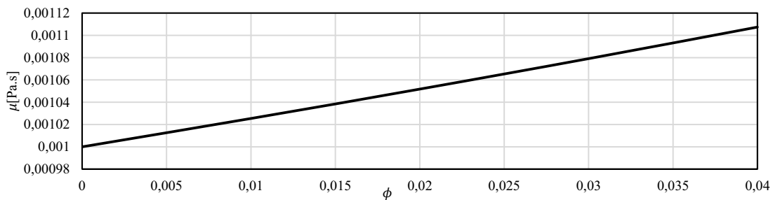
Figure 4. The effect of nanoparticles on the viscosity
