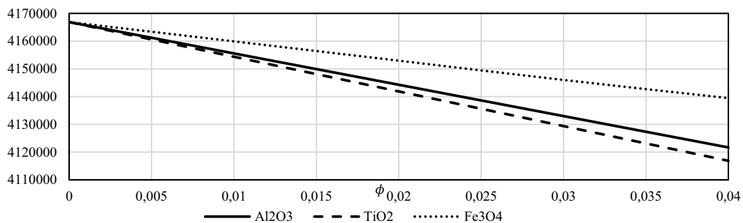
Figure 6. The effect of nanoparticles on (\rho C_p)
