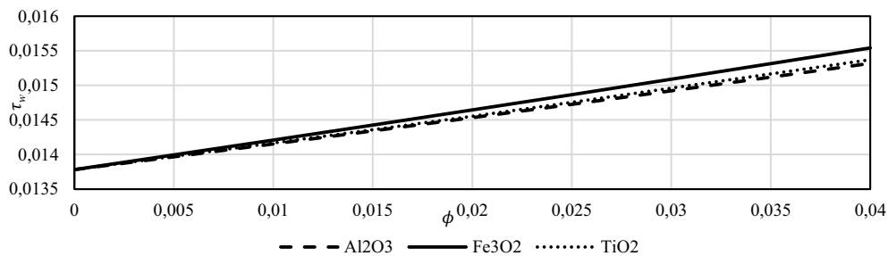
Figure 10. The wall shear stress vs volume fraction at x=0
