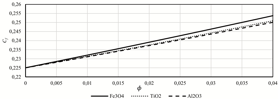
Figure 11. The effect of \phi on the skin friction coefficient
