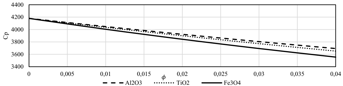
Figure 3. The effect of nanoparticles on the thermal capacity
