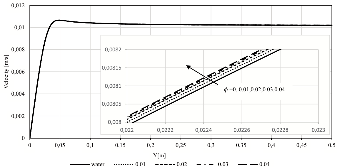
Figure 12. The effect of nanoparticles on the velocity profiles (Al 2 O 3 . water case)
