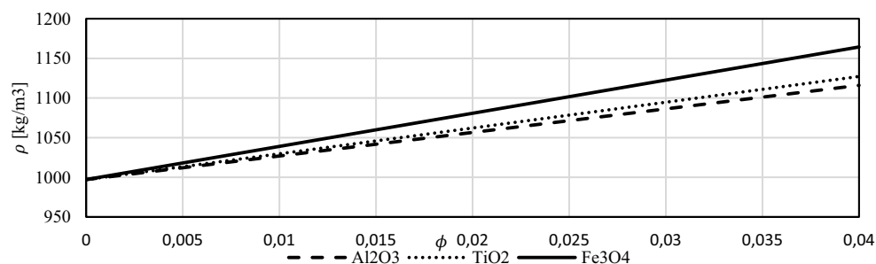
Figure 2. The effect of nanoparticles on the density
