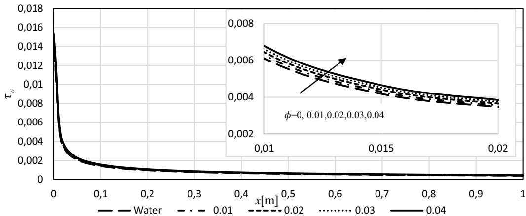
Figure 9. The effect of Al_2O_3 nanoparticles on the wall shear stress
