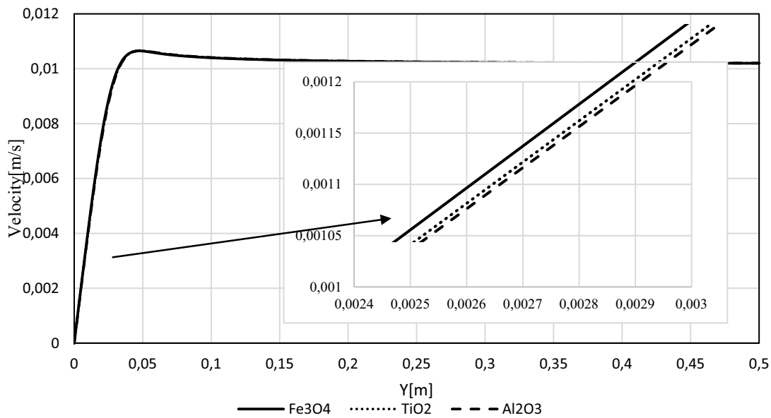
Figure 13. The velocity profile for different nanofluids for \phi = 0.04
