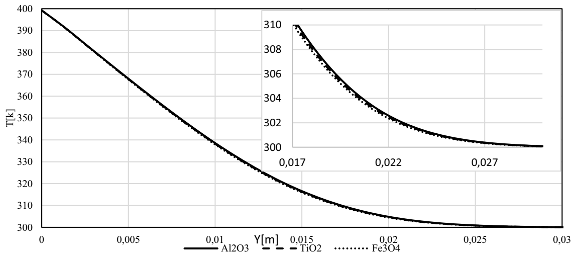
Figure 15. Comparison of the temperature for water based nanofluids with different nanoparticles ( \phi = 0.04 )
