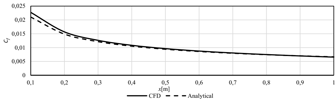
Figure 7. Skin friction comparison (water)
