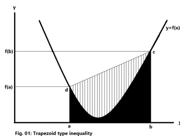
Fig. 01: Trapezoid type inequality
