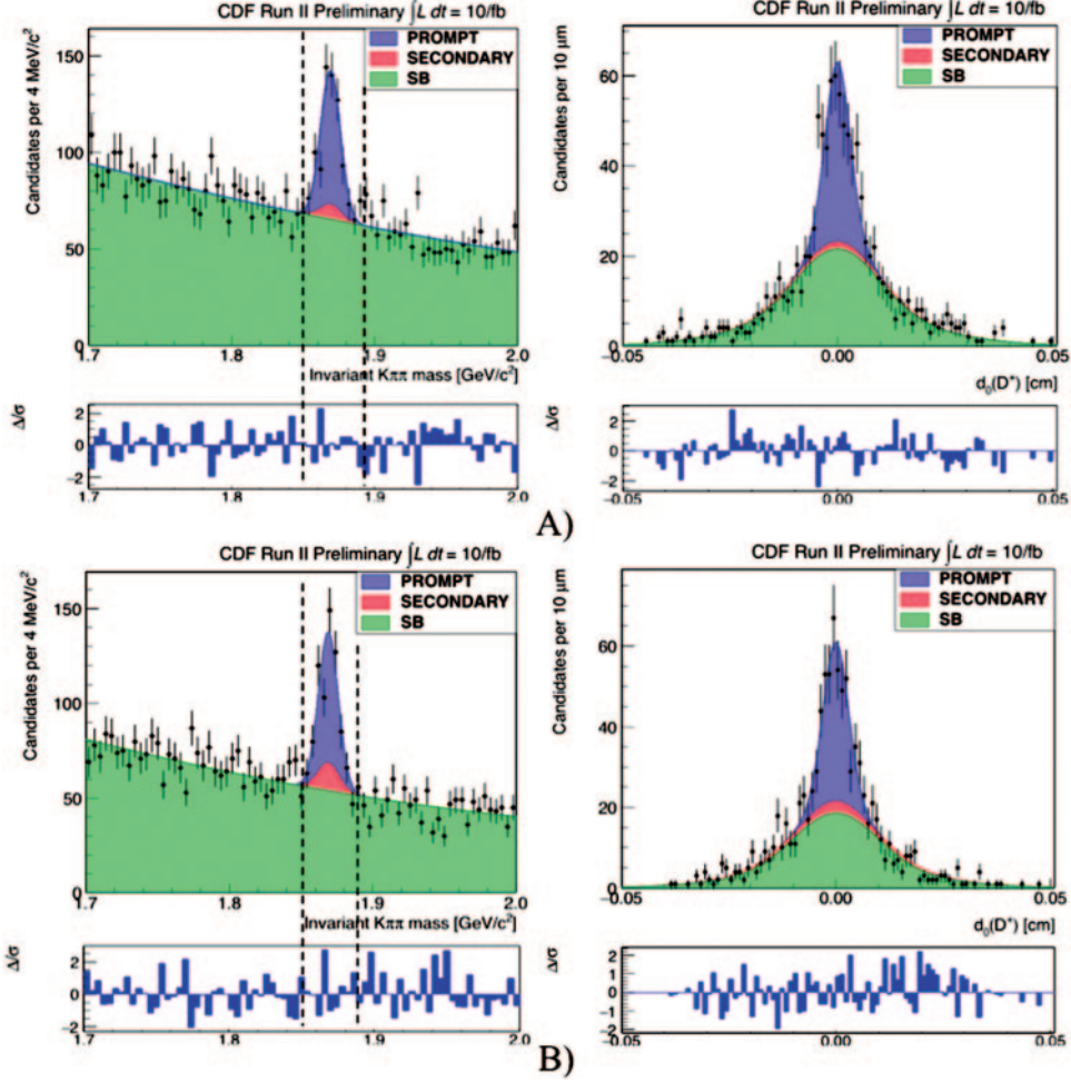
Fig. 2. – Two-dimensional unbinned likelihood fit for p_T(D^+) in the range [3.5; 4.5] GeV/ c for the even subsample A) and odd subsample B). On the left the results of the fit to the invariant mass distribution are shown, on the right the projection on the impact-parameter axis of the fit function in the signal region.
