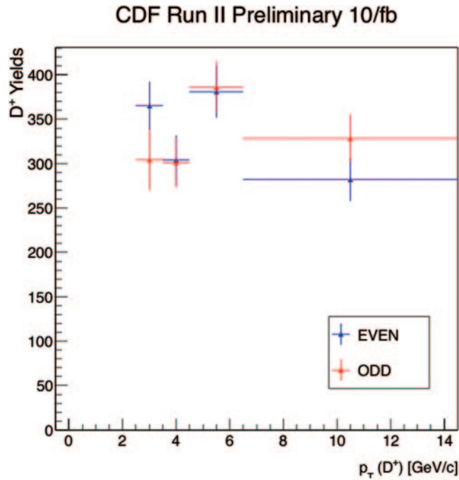
Fig. 5. – D^+ yields as a function of p_T .
