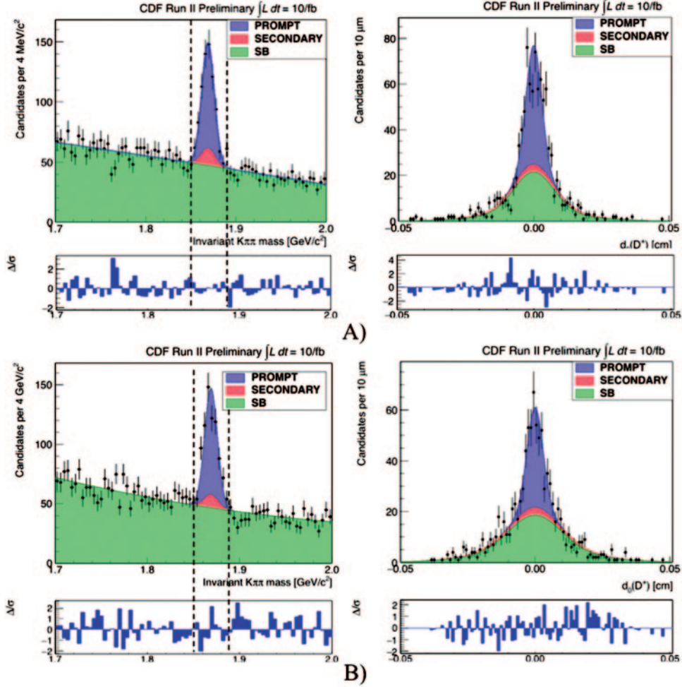
Fig. 3. – Two-dimensional unbinned likelihood fit for p_T(D^+) in the range [4.5; 6.5] \text{GeV}/c for the even subsample A) and odd subsample B). On the left the results of the fit to the invariant mass distribution are shown, on the right the projection on the impact-parameter axis of the fit function in the signal region.
