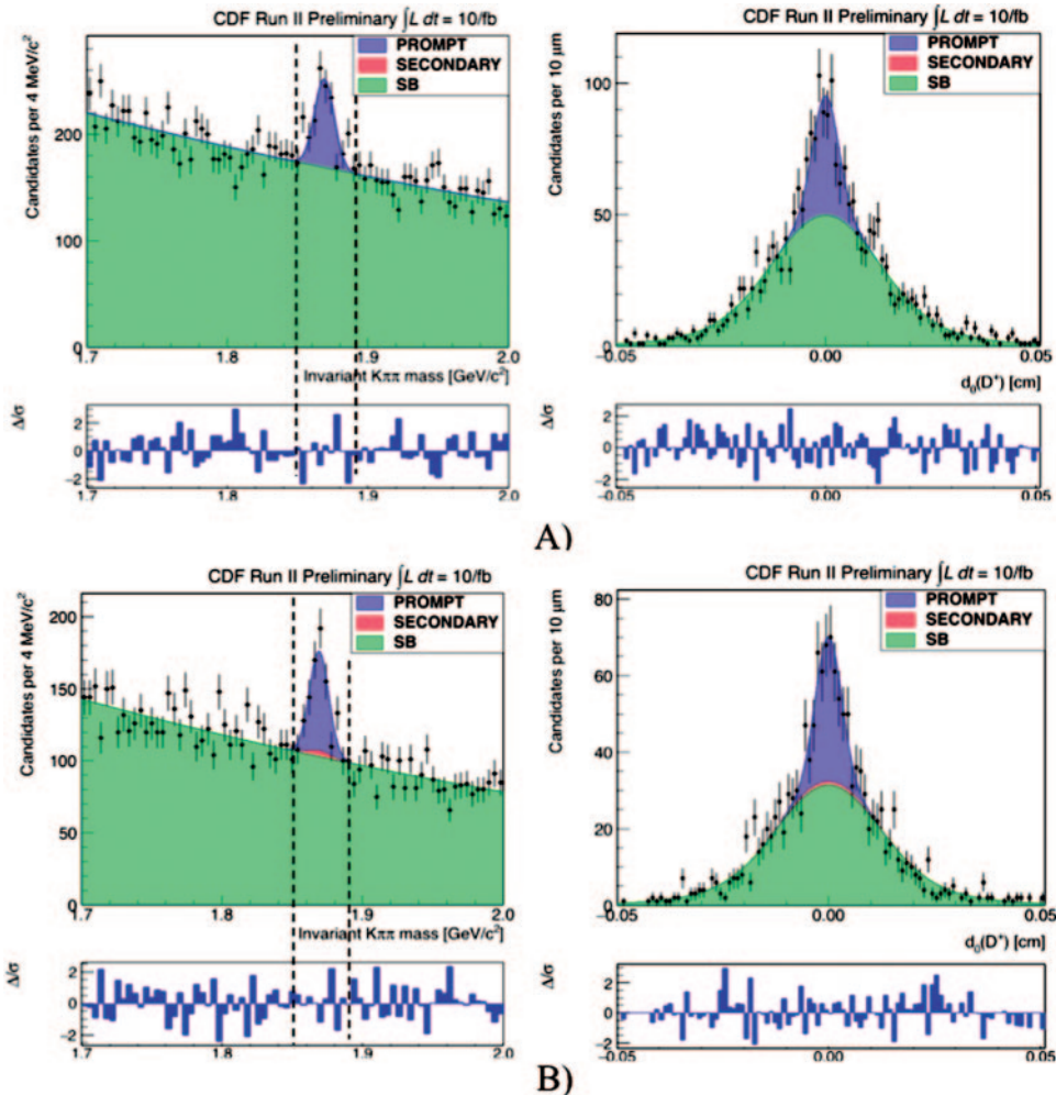
Fig. 1. – Two-dimensional unbinned likelihood fit for p_T(D^+) in the range [2.5; 3.5] \text{GeV}/c for the even subsample A) and odd subsample B). On the left the results of the fit to the invariant-mass distribution are shown, on the right the projection on the impact-parameter axis of the fit function in the signal region.
