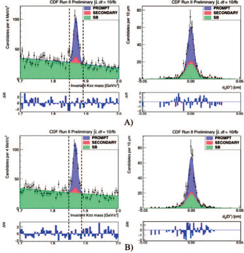
Fig. 4. – Two-dimensional unbinned likelihood fit for p_T(D^+) in the range [6.5; 14.5] \text{GeV}/c for the even subsample A) and odd subsample B). On the left the results of the fit to the invariant mass distribution are shown, on the right the projection on the impact-parameter axis of the fit function in the signal region.
