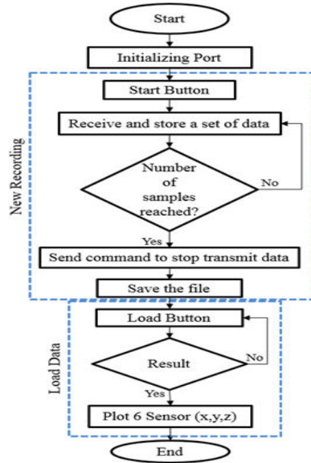
Figure-8. Flowchart of MATLAB for displaying.
