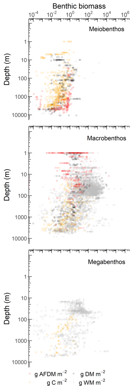
Fig. 5 Benthic biomasses ( \text{g m}^{-2} ) of metazoan meiobenthos (upper panel), macrobenthos (middle panel), and invertebrate megabenthos (lower panel) along a water depth gradient (m). Note the logarithmic scale on both axes. Abbreviations: AFDM = ash-free dry mass, DM = dry mass, C = carbon, WM = wet mass.
